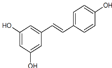
Obr. 14: Resveratrol
