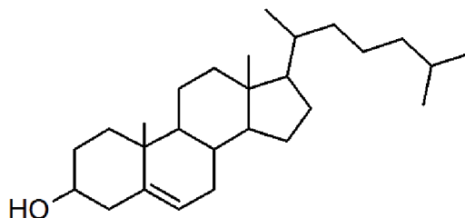
Obr. 9: Cholesterol
