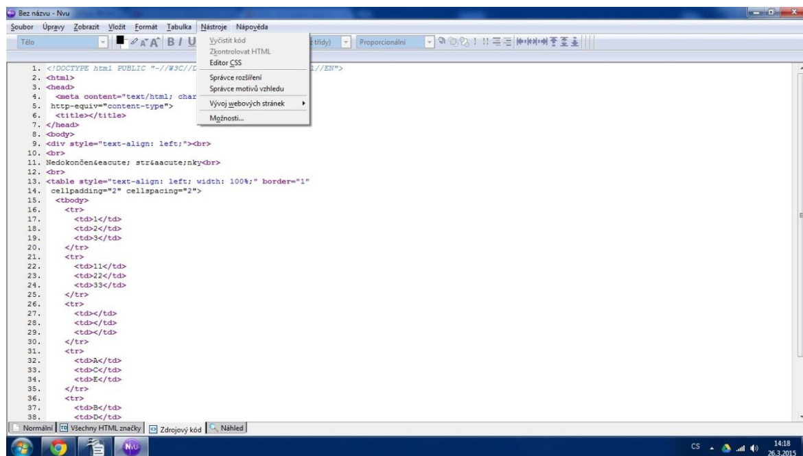
Obr. 10: Program Nvu 1.0
