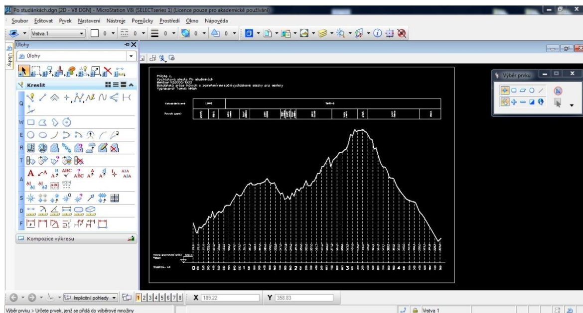
Obr. 5: Microstation V8i
