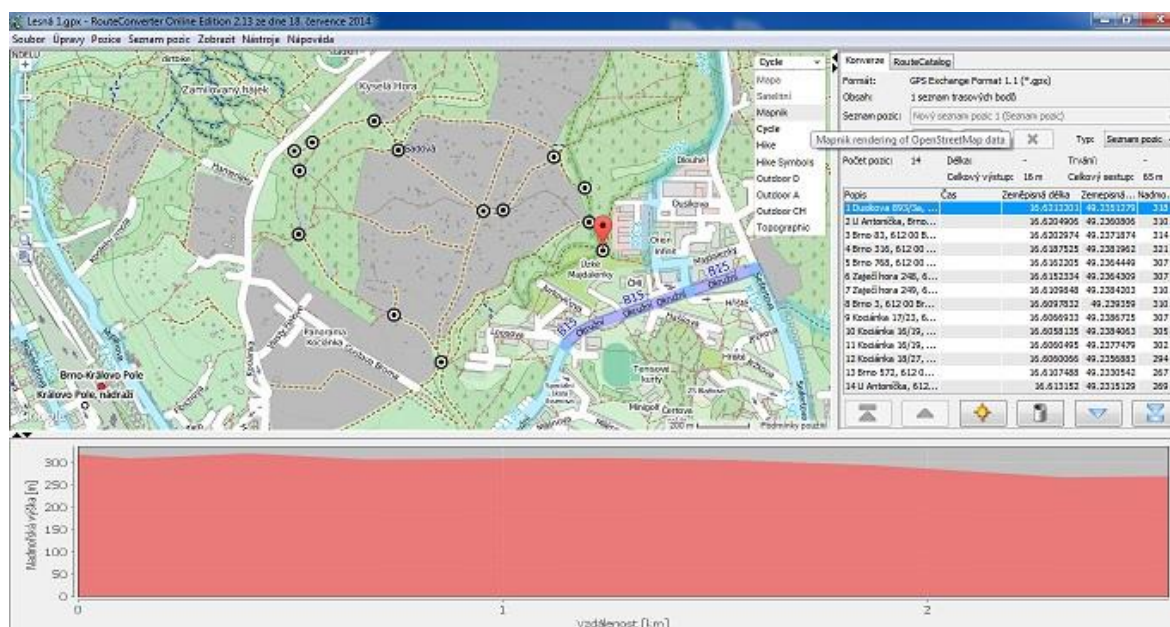
Obr. 2: Program RouteConverter
