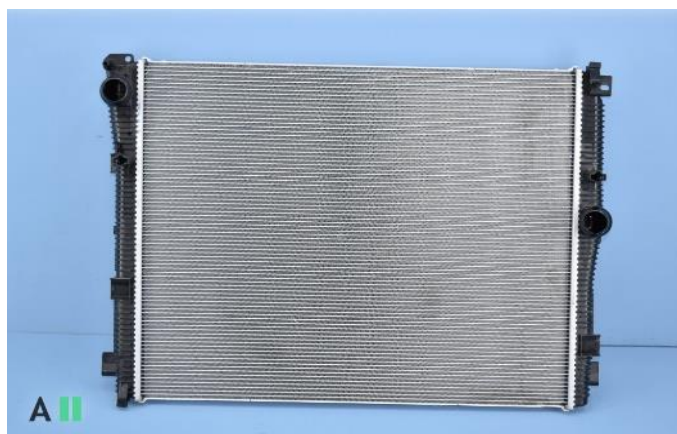
Obr. 15 Chladič BMW iX xDrive50 Sport 2022 [13]
