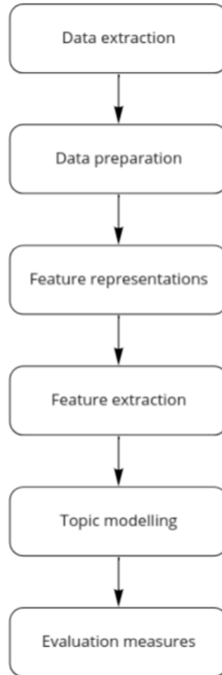
Figure 4.1: Process Pipeline
