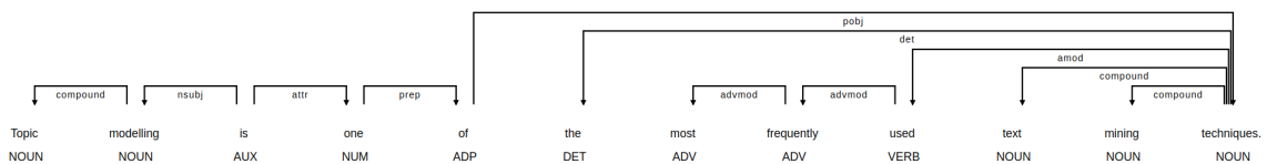
Figure 3.2: Dependency Structure
