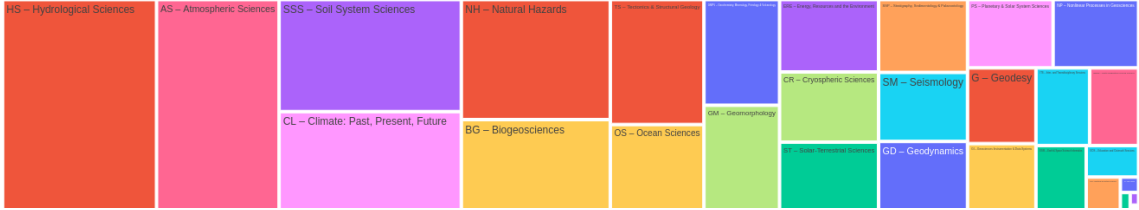
Figure 4.2: Sessions Division
