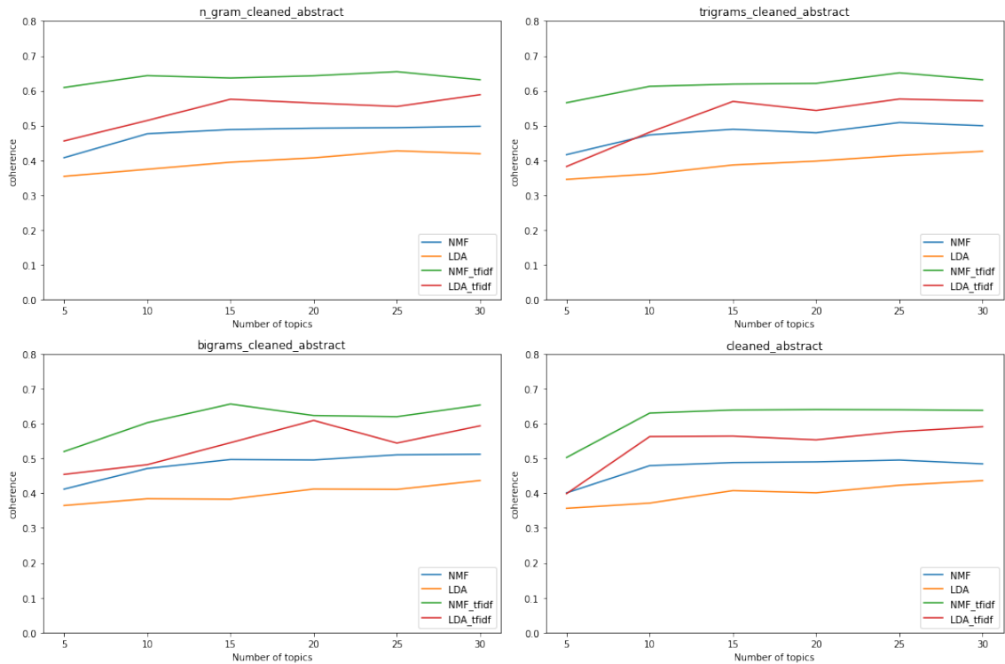
Figure 5.5: Coherence measure
