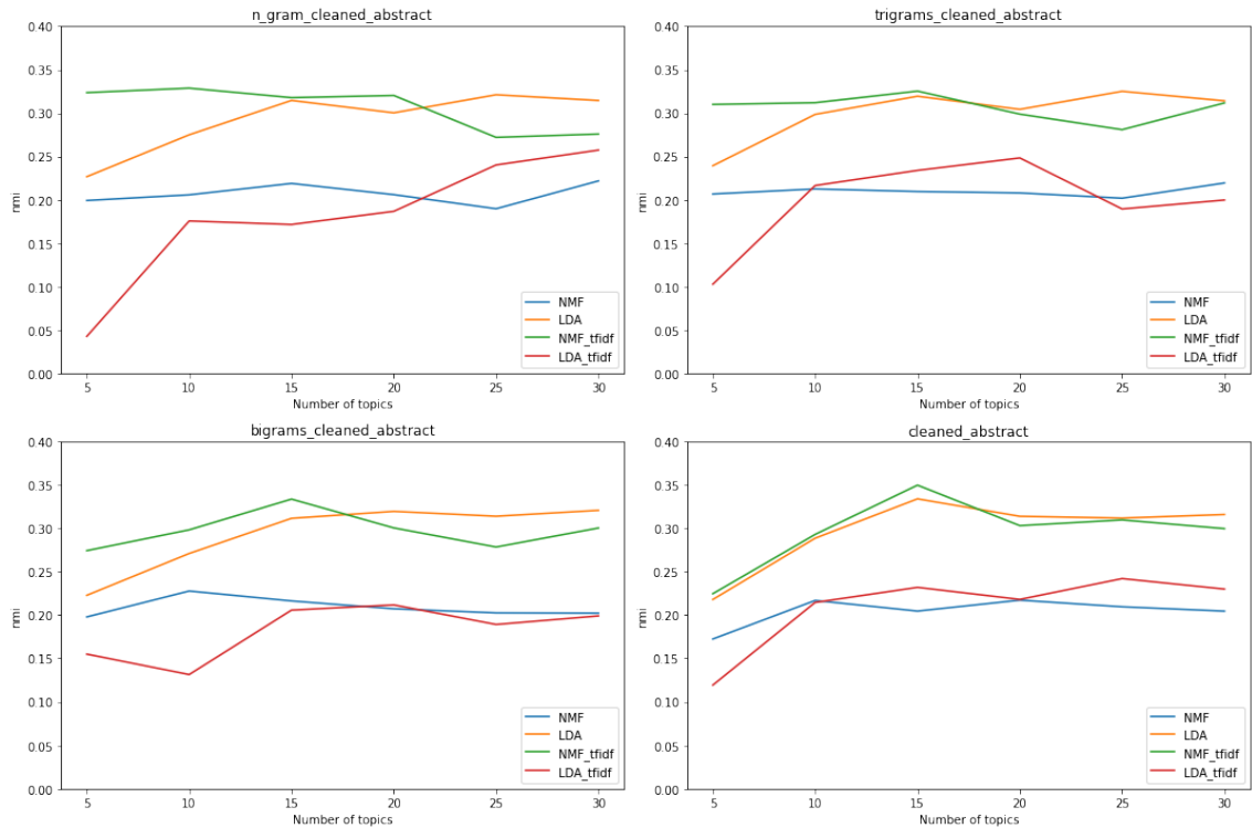
Figure 5.7: NMI measure
