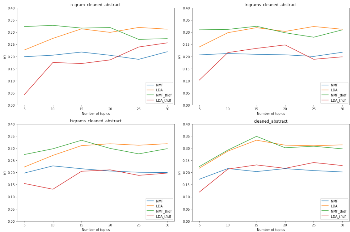
Figure 5.8: ARI measure
