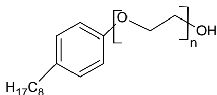
Obr. 16: 4-(1,1,3,3-Tetramethylbutyl)fenyl-polyethylen glykol (Triton X-100)
