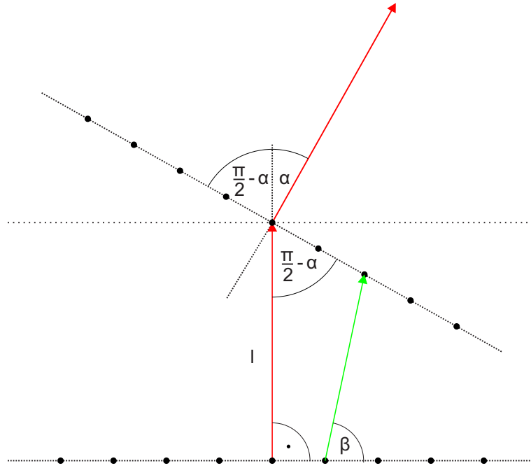
Figure 6.6: A relation between two vectors used during the fitness evaluation
