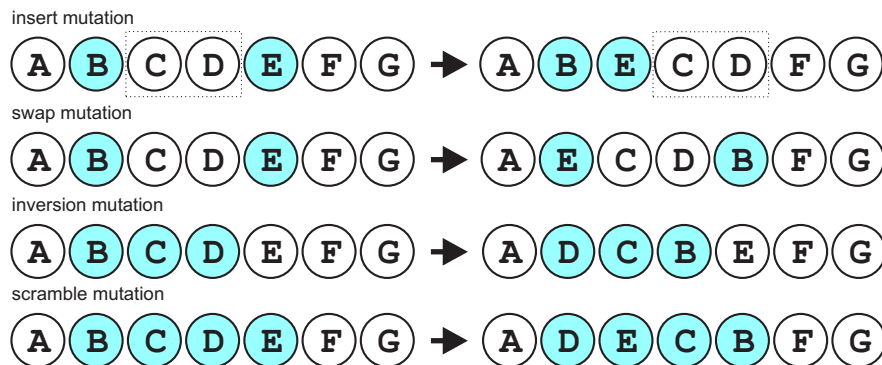
Figure 4.10: Permutation mutations
