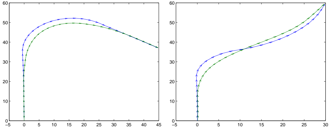
Figure 8.7: Optimized segments of the Aalborg track
