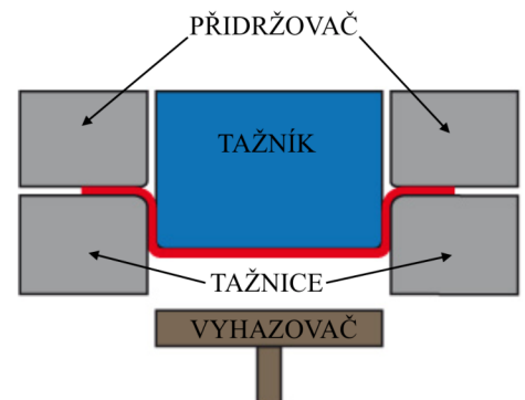
Obr. 8 Schéma Hydroform [11]
