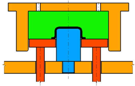
Obr. 7 Schéma Marform [20]
