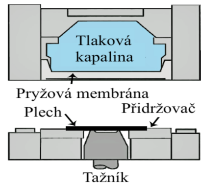
Obr. 8 Schéma Hydroform [11]
