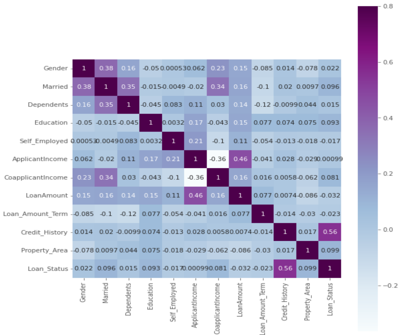
Figure 34: Correlation heatmap for understanding relationship between variables.
