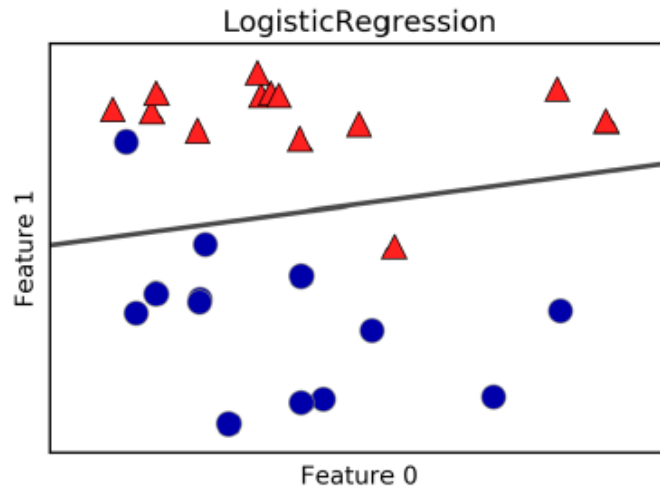
Figure 16: Example of decision boundary of a logistic regression on the dataset.[26]
