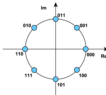
Obr. 3.12: D8PSK
