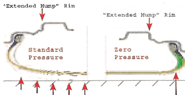
Obr. 8.5 Pirelli PTM
