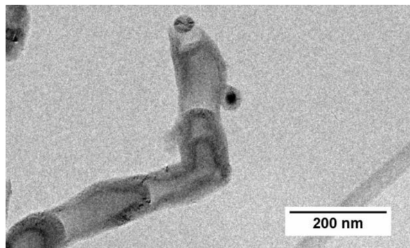
Fig. 4.10: TEM observed for suspended BNNT in ethanol
