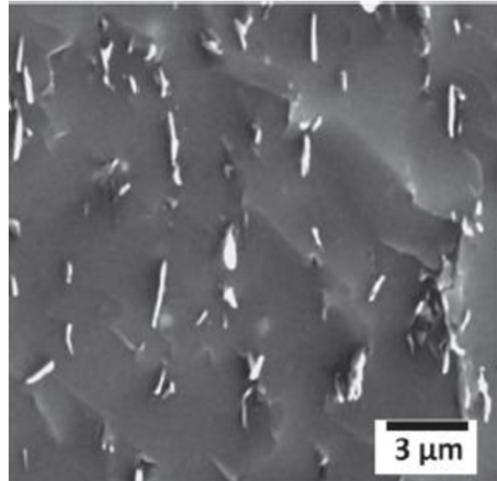
Fig. 2.7: Dispersion of 2.5 vol% of graphene in silica matrix by powder processing 14
