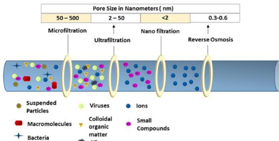
Figure 2. Categories of membrane separation methods and their efficiency of molecules (Rezakovski et al., 2018)
