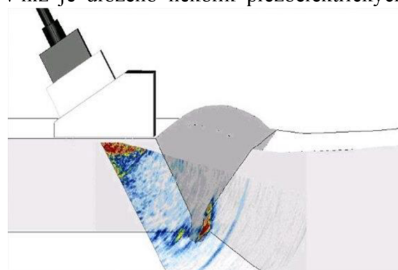
Obr. 17 Phased Array technika [28]
