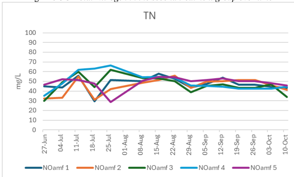
Figure 5.3.4. Total Nitrogen in the third treatment group over time
