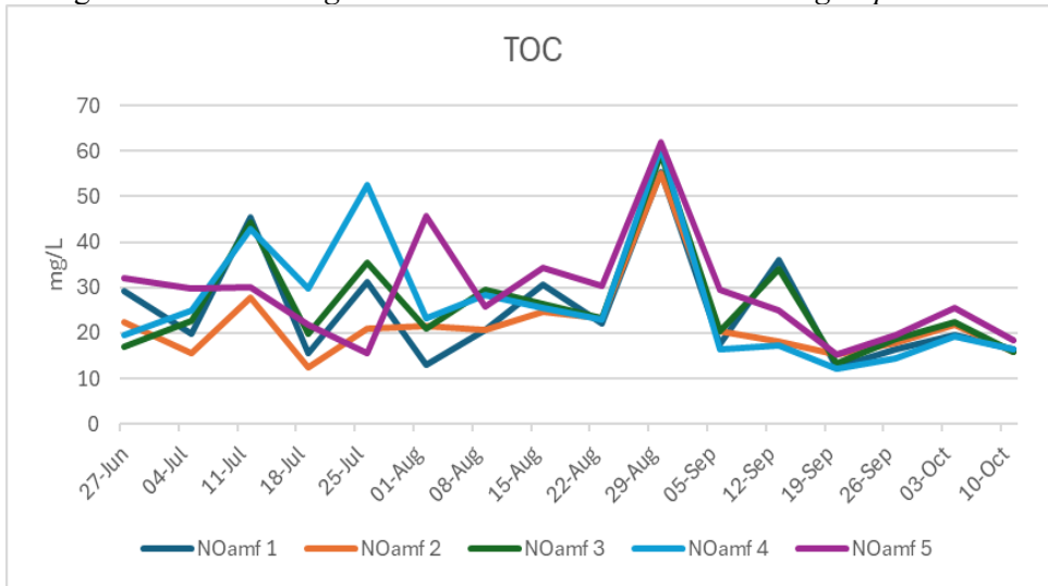
Figure 5.5.4. Total Organic Carbon in the third treatment group over time
