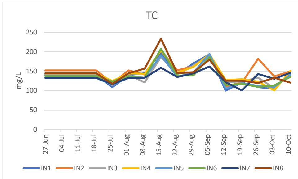
Figure 5.4.1. Total Carbon in the inflow group over time
