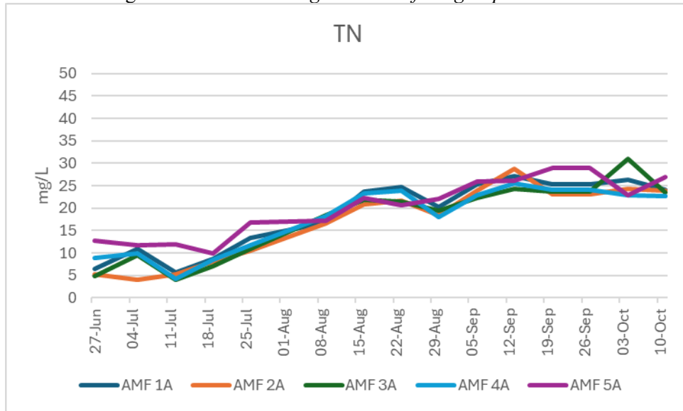
Figure 5.3.2. Total Nitrogen in the first treatment group over time
