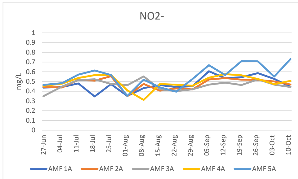
Figure 5.2.11 Nitrites in the inflow group over time
