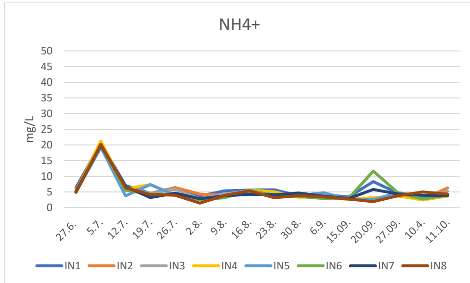
Figure 5.2.1. Ammonium in the inflow group over time
