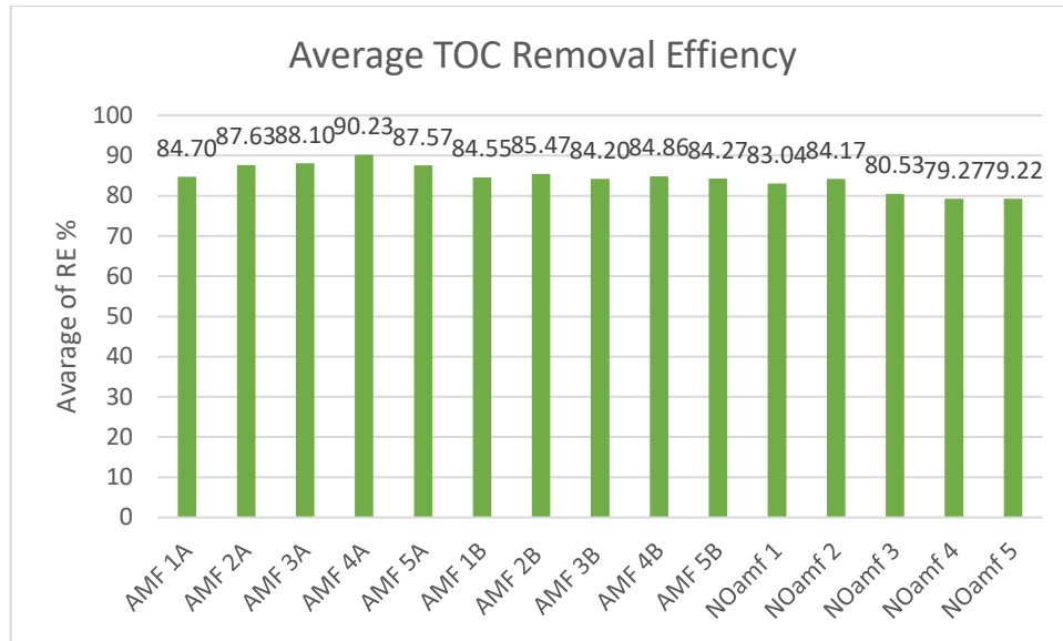
Figure 5.5.5 Average of Total Organic Carbon Removal Efficiency
