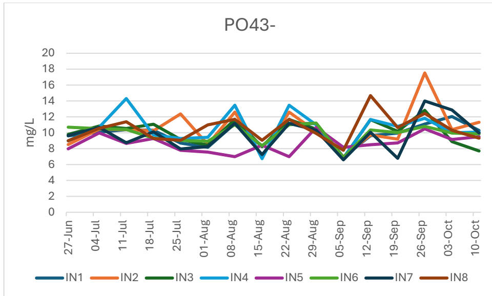
Figure 5.2.14 Phosphates in the inflow group over time
