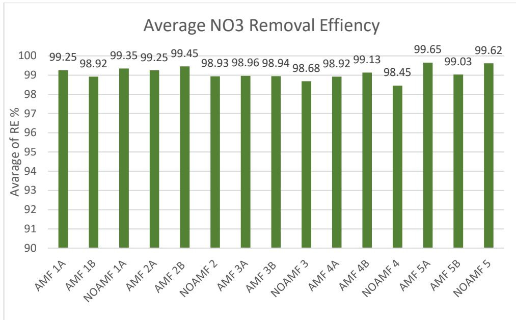
Figure 5.2.8 Average of Nitrates Removal Efficiency
