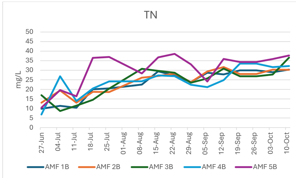
Figure 5.3.3. Total Nitrogen in the second treatment group over time
