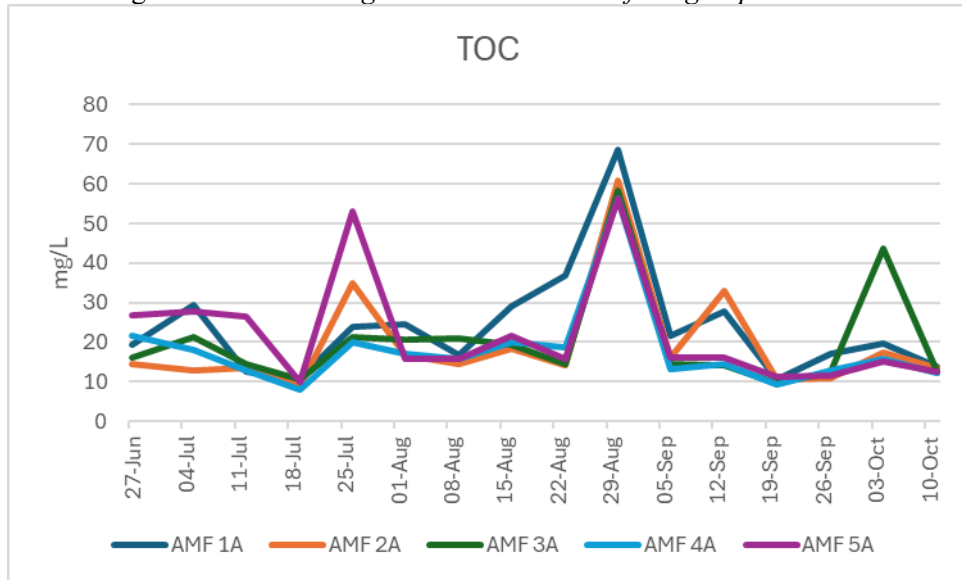
Figure 5.5.2. Total Organic Carbon in the first treatment group over time
