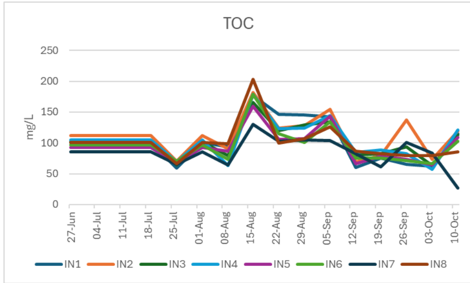
Figure 5.5.1. Total Organic Carbon in the inflow group over time
