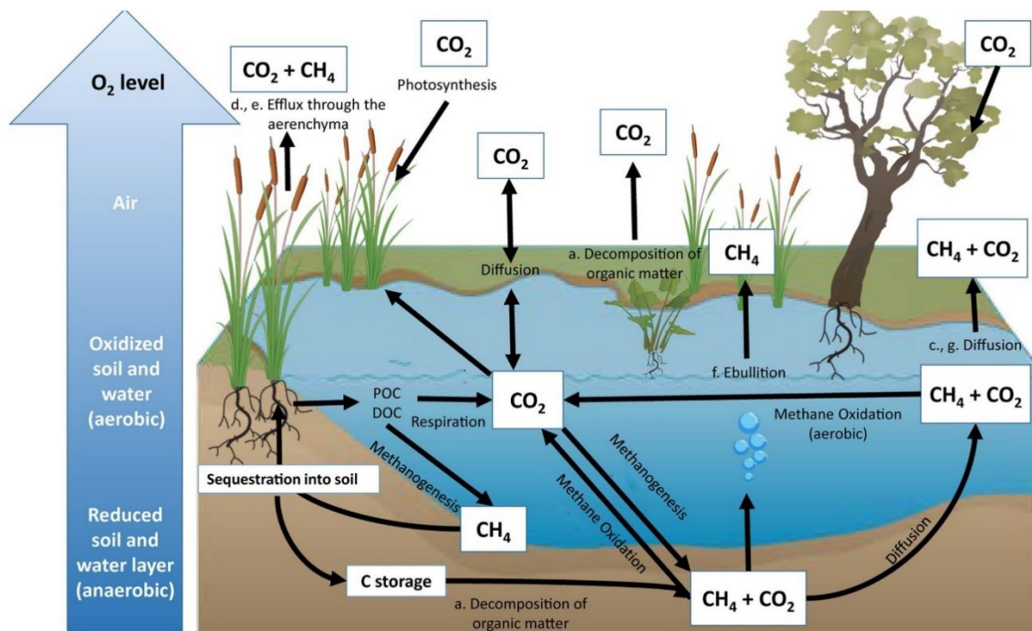
FIGURE 3.5.2. Representation of the inland wetland carbon cycle. Major pathways of carbon sequestration include photosynthesis and organic carbon accumulation (Bernal and Mitsch, 2012)
