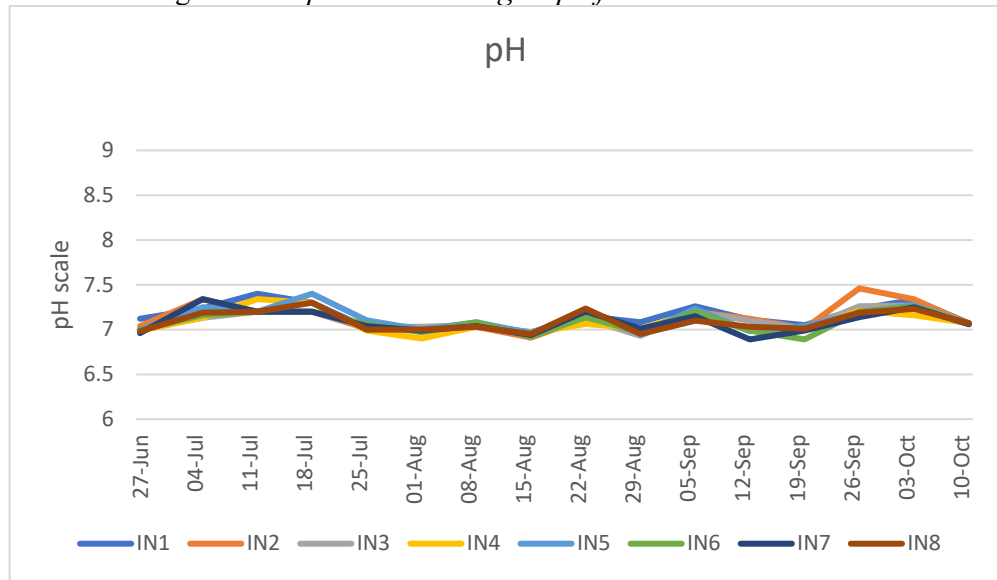
Figure 5.1.7. pH in the inflow group of treatment over time
