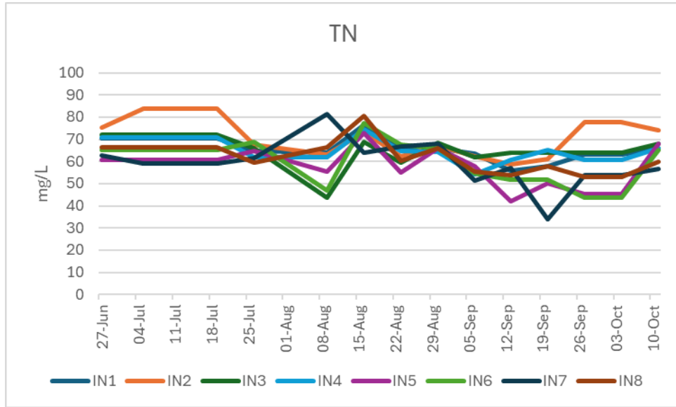
Figure 5.3.1. Total Nitrogen in the inflow group over time
