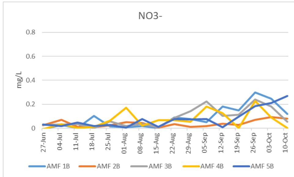
Figure 5.2.6 Nitrates in the second treatment group over time
