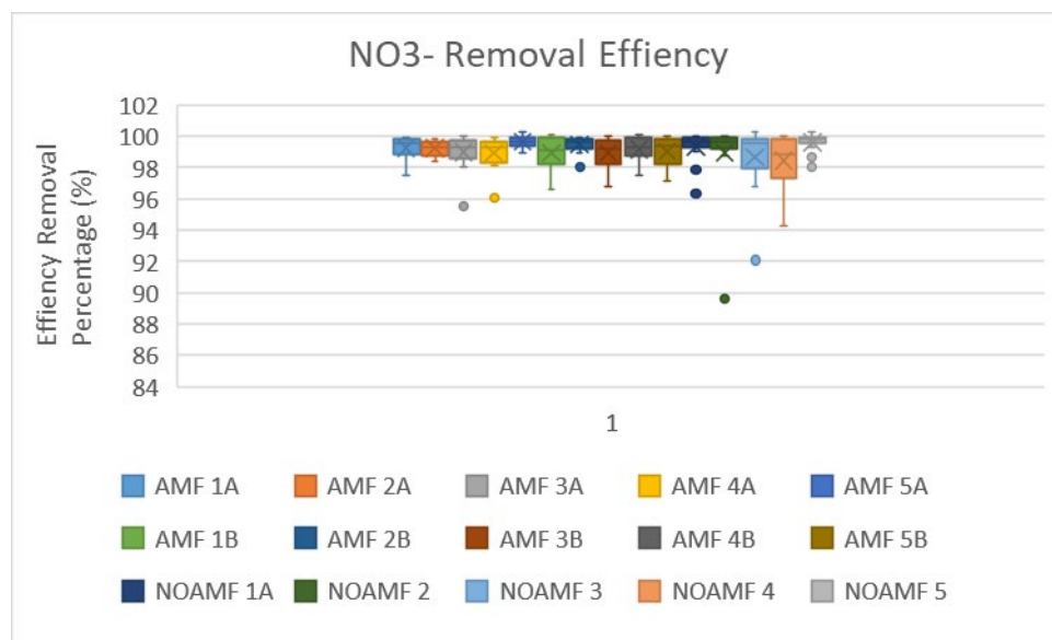
Figure 5.2.9 Variation of Nitrates Removal Efficiency
