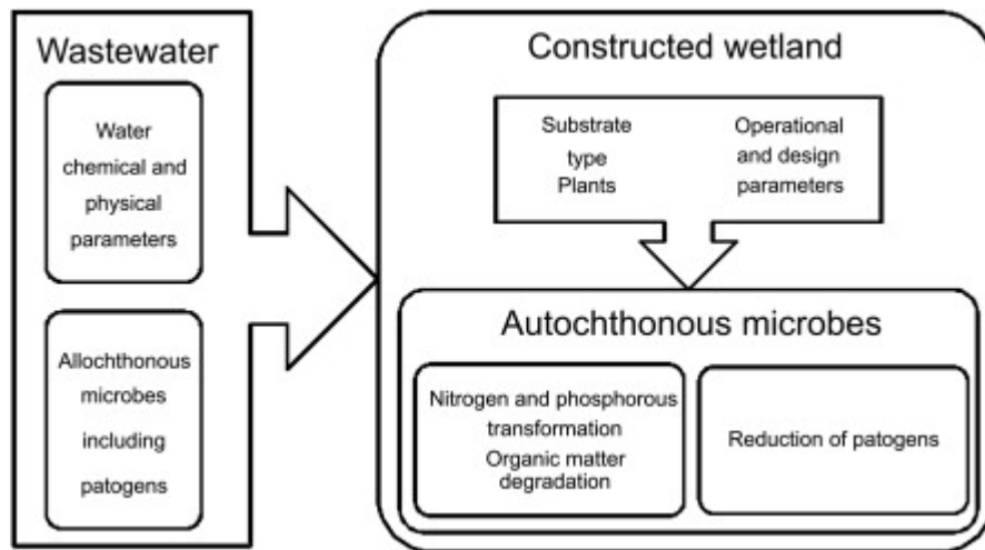
Figure N°3.6.1. External and internal factors which may affect microbial community structure and activity in constructed wetlands. (Truu et al., 2009).
