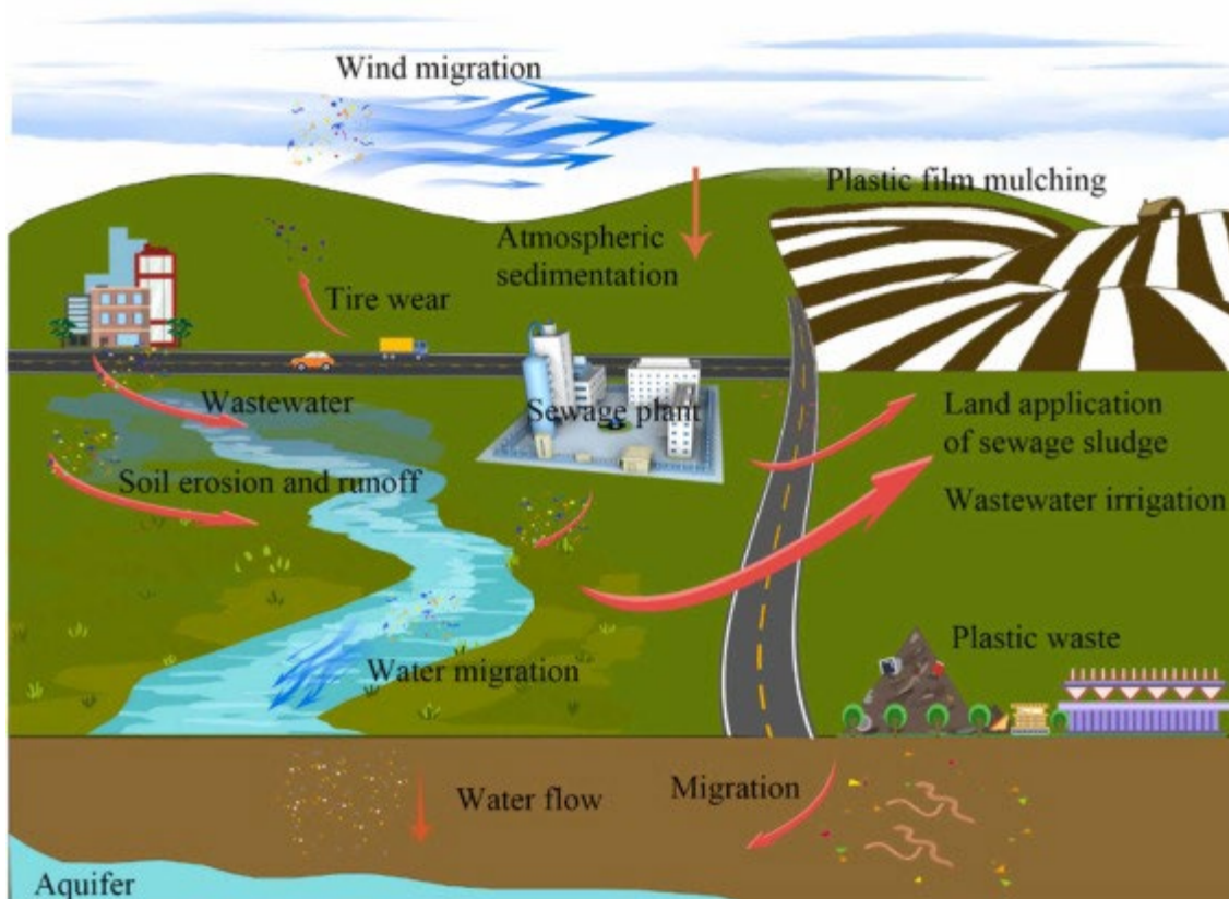
Fig. 3.8.1. Potential sources and migration of MPs in the soil. (Wang F. et al., 2022)
