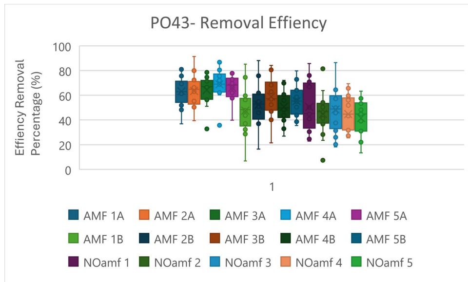
Figure 5.2.19 Variation of Phosphate Removal Efficiency
