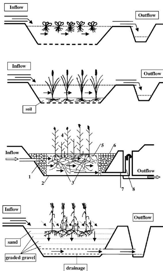
Figure N°3.2.2 -From Top to bottom - CW with free-floating plants (FFP), CW with free water surface and emergent macrophytes (FWS), CW with the horizontal sub-surface flow (HSSF, HF), CW with the vertical sub-surface flow (VSSF, VF). (Vymazal,2001)
