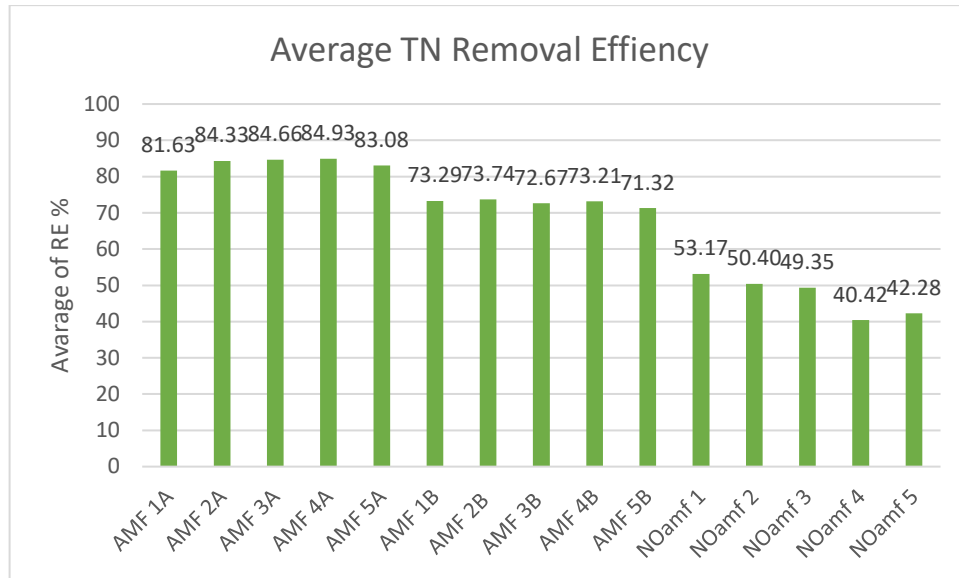
Figure 5.3.5 Average of Total Nitrogen Removal Efficiency
