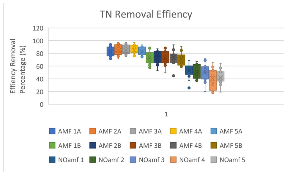
Figure 5.3.6 Variation of Total Nitrogen Removal Efficiency
