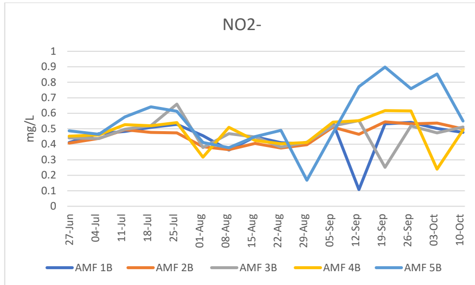
Figure 5.2.12 Nitrites in the second group over time
