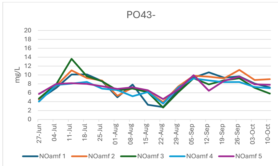
Figure 5.2.17 Phosphates in the third group over time
