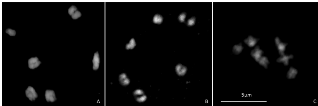
Fig. 2. Meiosis in B+ plants of Sorghum purpureosericum . (A) B+ plant ( 2n=2x=10+B ) forming five bivalents and one univalent in meiotic metaphase I; (B) B+ plant ( 2n=2x=10+2B ) showing six ring bivalents; and (C) B+ plant ( 2n=2x=10+4B ) with seven bivalents.
