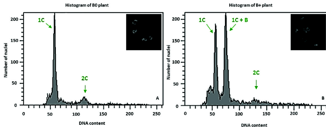
Fig. 1. Flow histograms of pollen nuclei isolated from B0 (A) and B+ (B) plants of Sorghum purpureosericum . Insets show the number of bivalents in meiotic metaphase I of analysed plants. (A) Histogram of a B0 plant with two peaks representing haploid 1C pollen nuclei and 2C nuclei corresponding to residual cells from tapetum. (B) The population of haploid cells splits into two distinct subpopulations representing those harbouring 1C and 1C+B nuclei.
