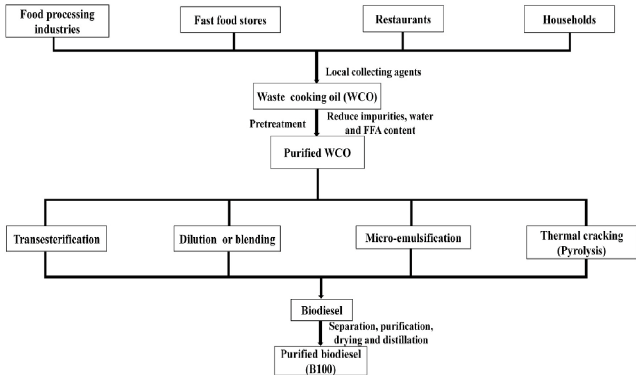
Figure 8 Illustrate processes for the production of biodiesel from WCO (Singh et al., 2020).
