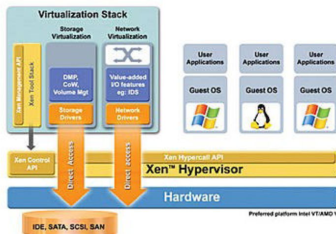
Obr. 15: Xen Hypervisor
