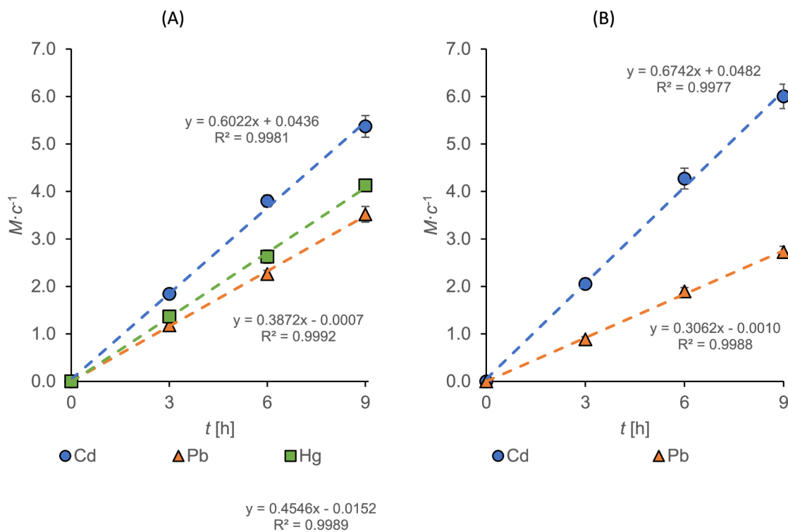
Fig. 3. Linear accumulation of Cd, Pb and Hg on S924-DGT (A) and Chelex-DGT (B) in fish sauce solution (5-fold diluted fish sauce sample 1, spiked to 50 \mu\text{g L}^{-1} of Hg, Cd and Pb with final NaCl concentration of 42 \text{ g L}^{-1} at pH 6).
