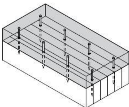
Upright special screws
