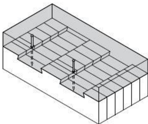
Bird's mouth joints and screws
