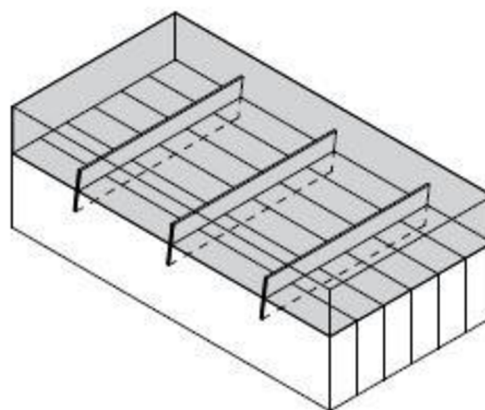
Flat steel elements set in sawn grooves
