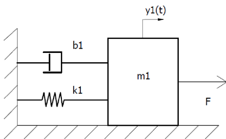
Fig. 5-7: Mass-spring-damper system 1
