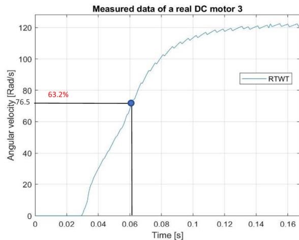
Fig. 6-9: Measured data of Tau Mechanical
