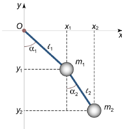
Fig. 5-13: Double pendulum
