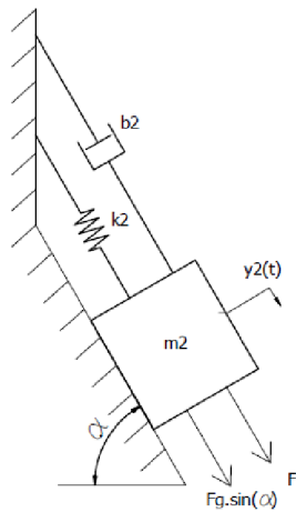
Fig. 5-9: Mass-spring-damper system 2
