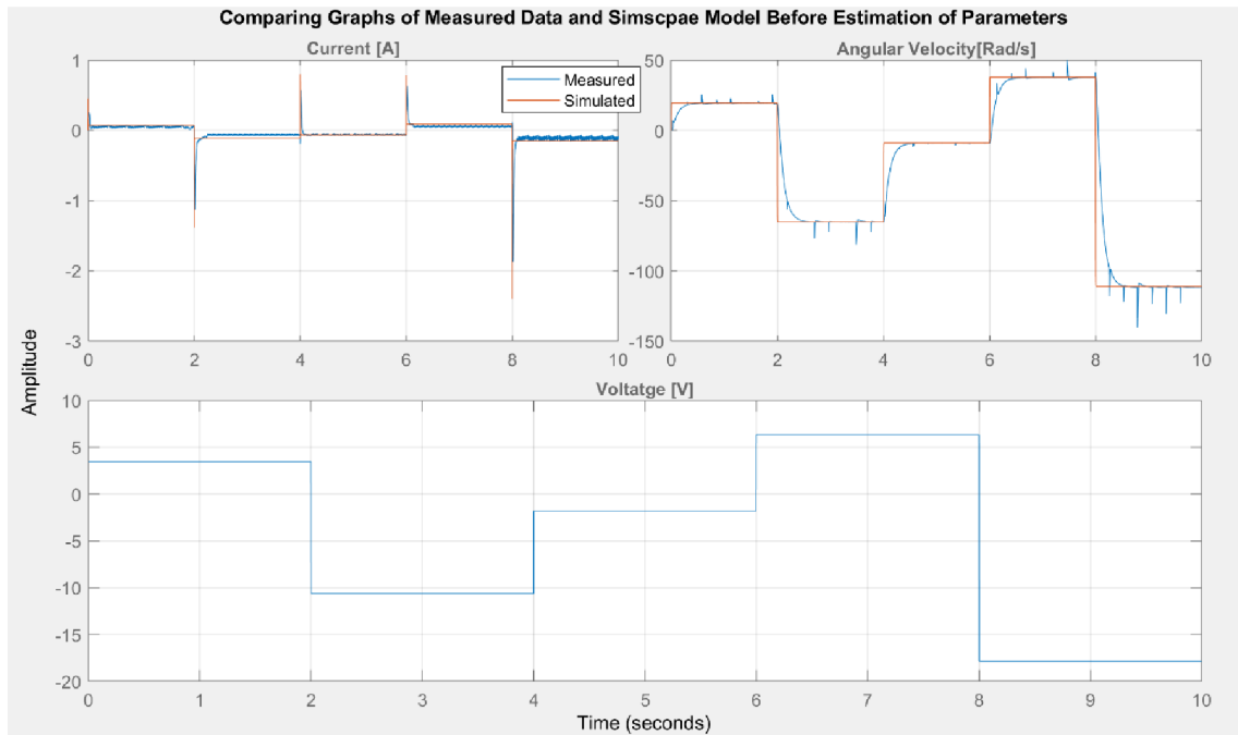
Fig. 6-11: Comparing Measured data graphs of angular velocity and current with graphs of DC Simscape model before Estimation
