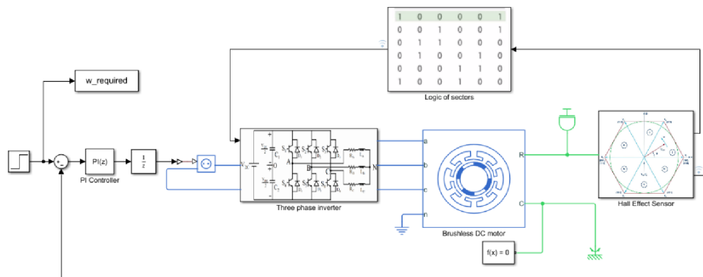
Fig. 5-4: BLDC Model
