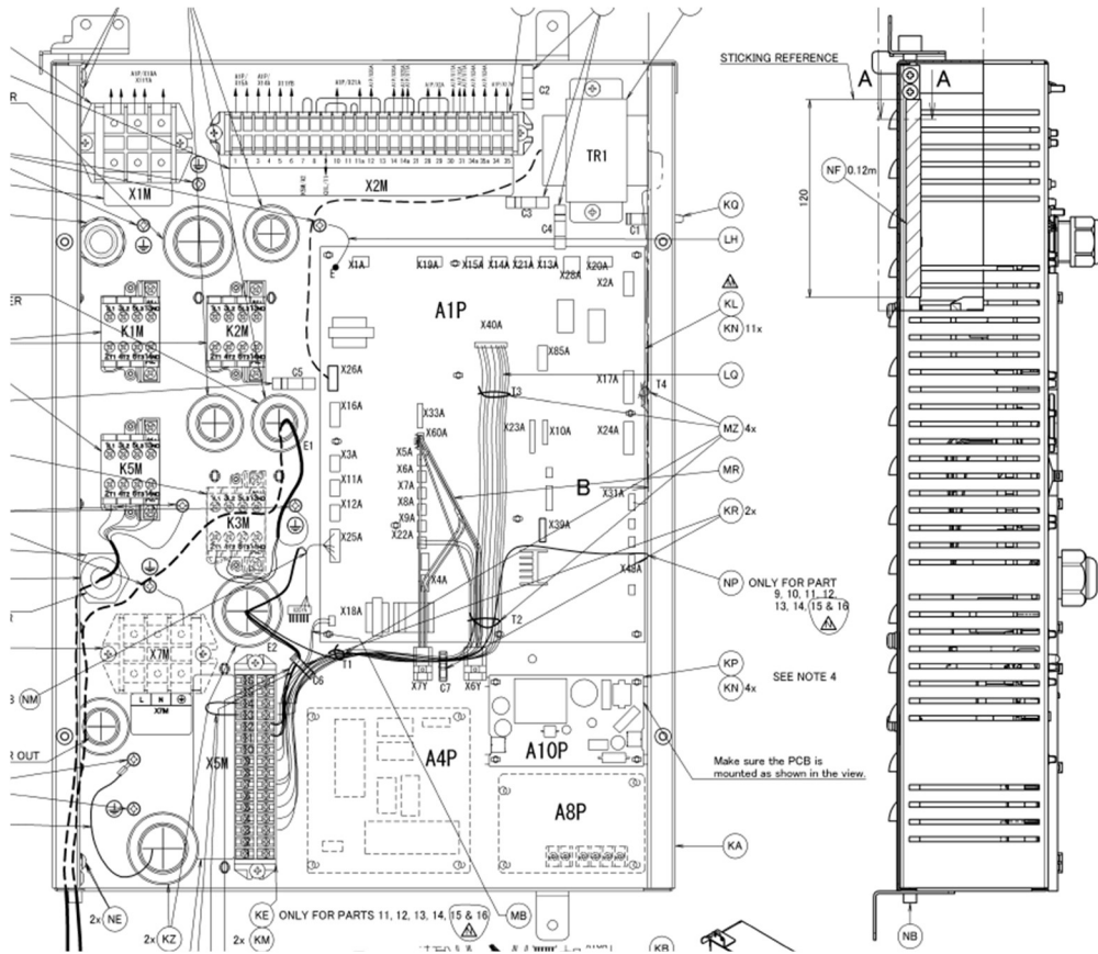
Obr. 5-3 Switchbox Altherma D/E series WM [20]
