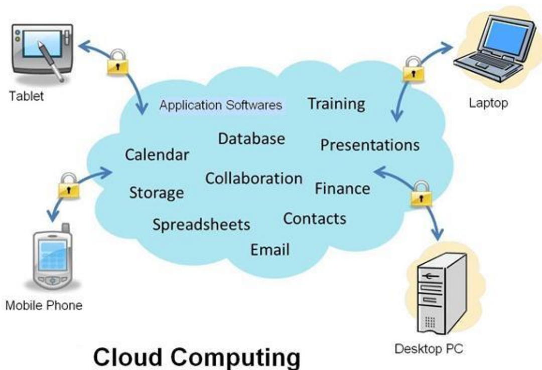
Obr. 1. Cloud Computing [4].
