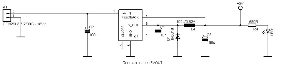
Regulace napeti 5VOUT
