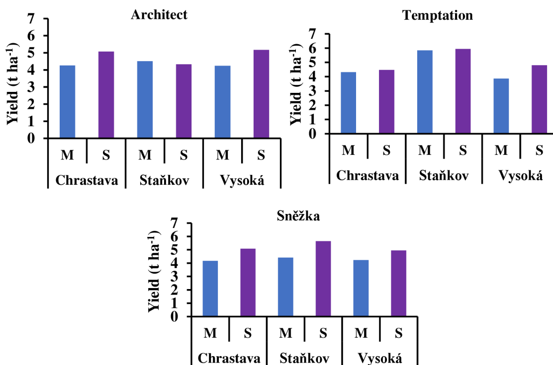
Figure 8. Observed and simulated yields of winter rape varieties for the 2020-2021 growing season. Yield is expressed as dry biomass per hectare (t ha -1 )
