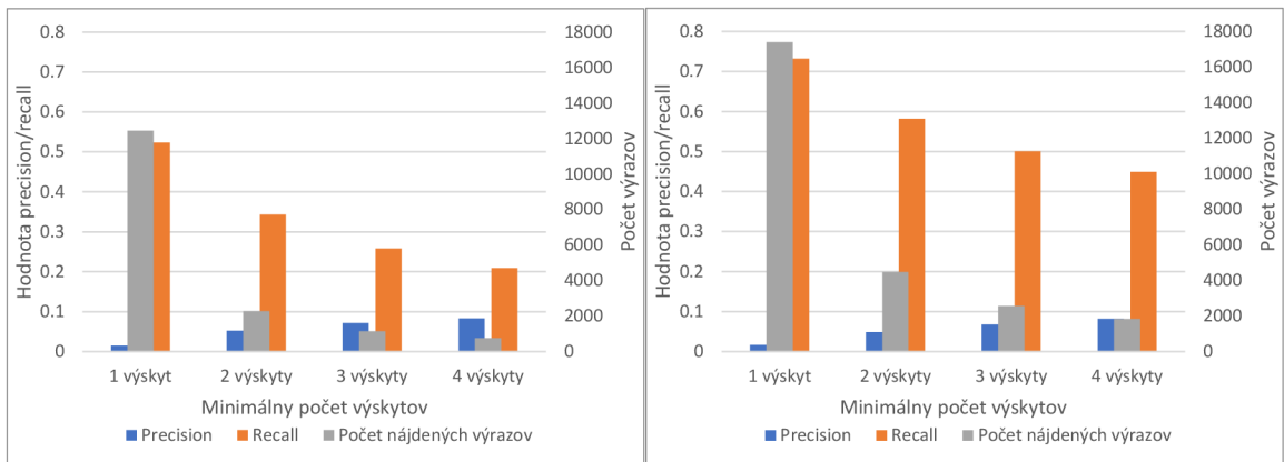
(a) RAKE
