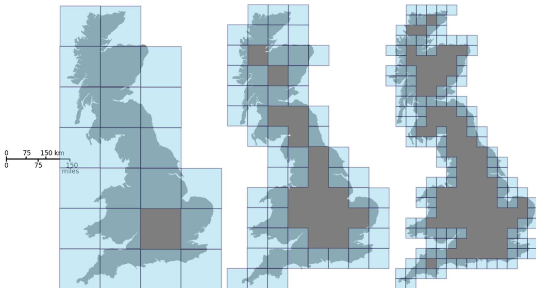
Obr. 11: Princip metody Box counting [9]
