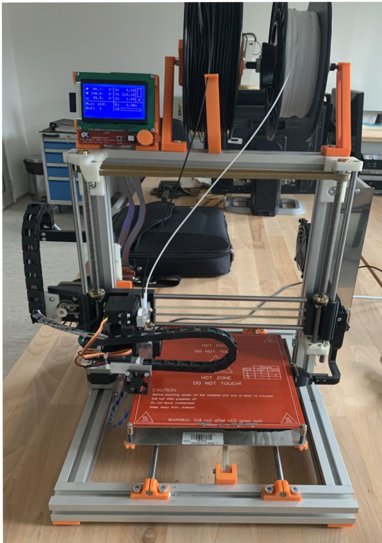
Figure 16: 3D Printer
