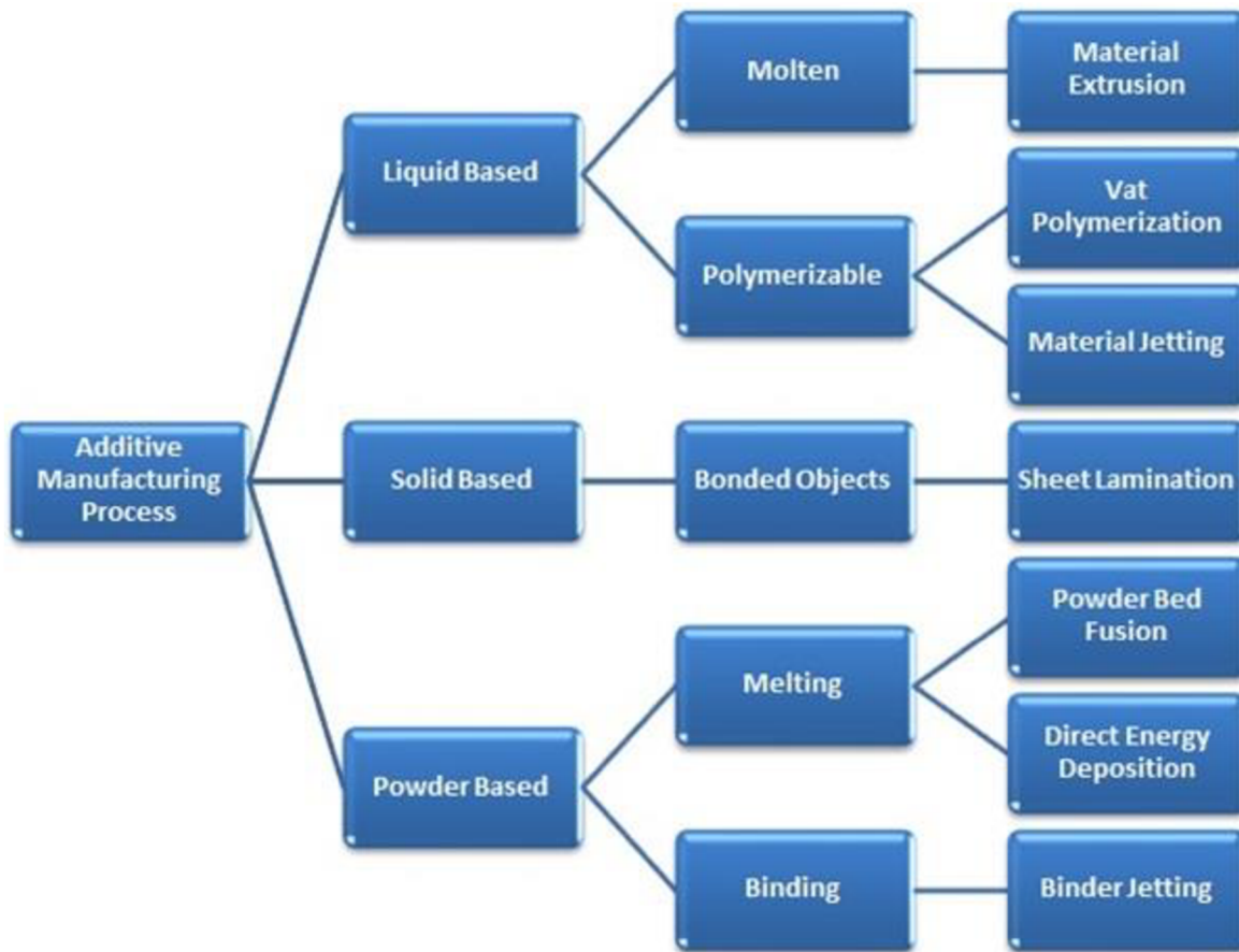
Figure 4: Additive Manufacturing technology[4]
