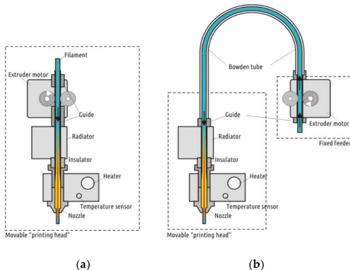
Figure 10: Direct drive and Bowden[7]
