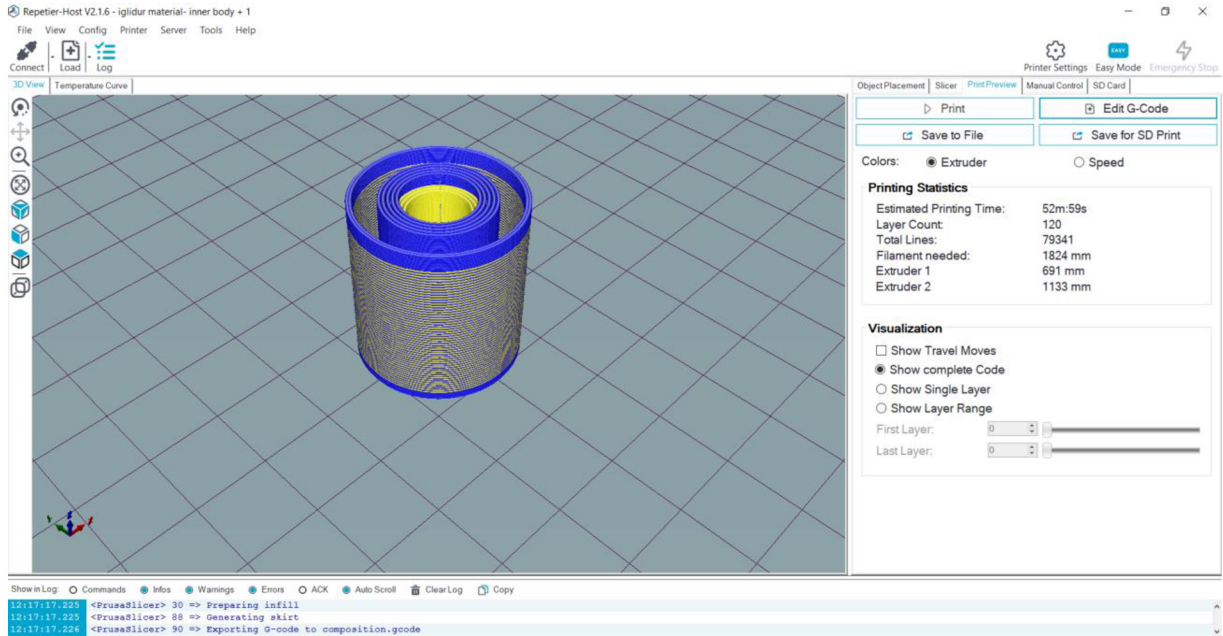
Figure 36: Printer Preview- With Ooze Shield
