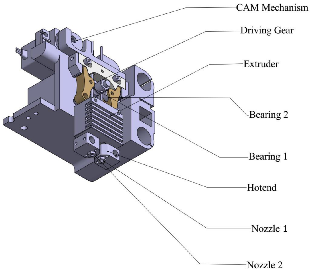
Figure 7: Material Extrusion
