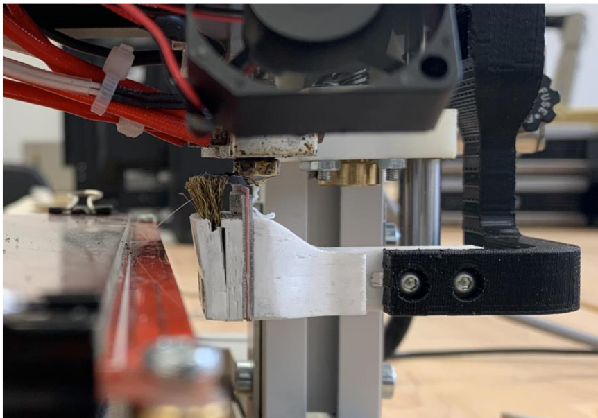
Figure 46: New brush and Rubber Holder
