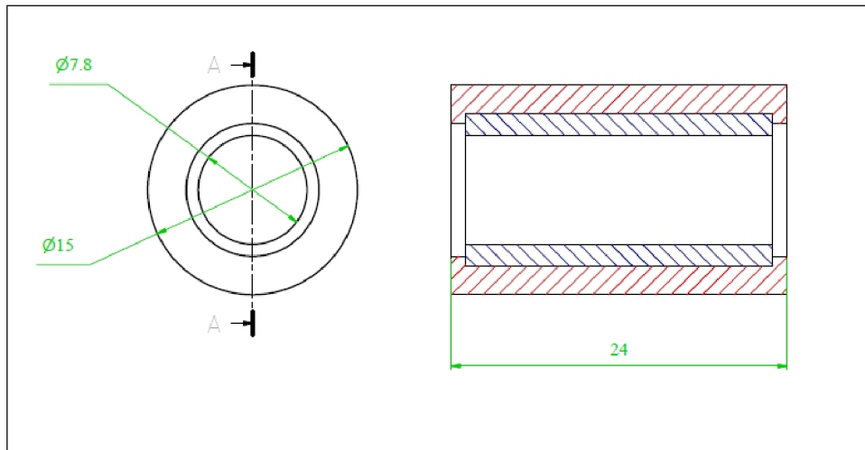
Figure 53: Linear Bearing Parameters
