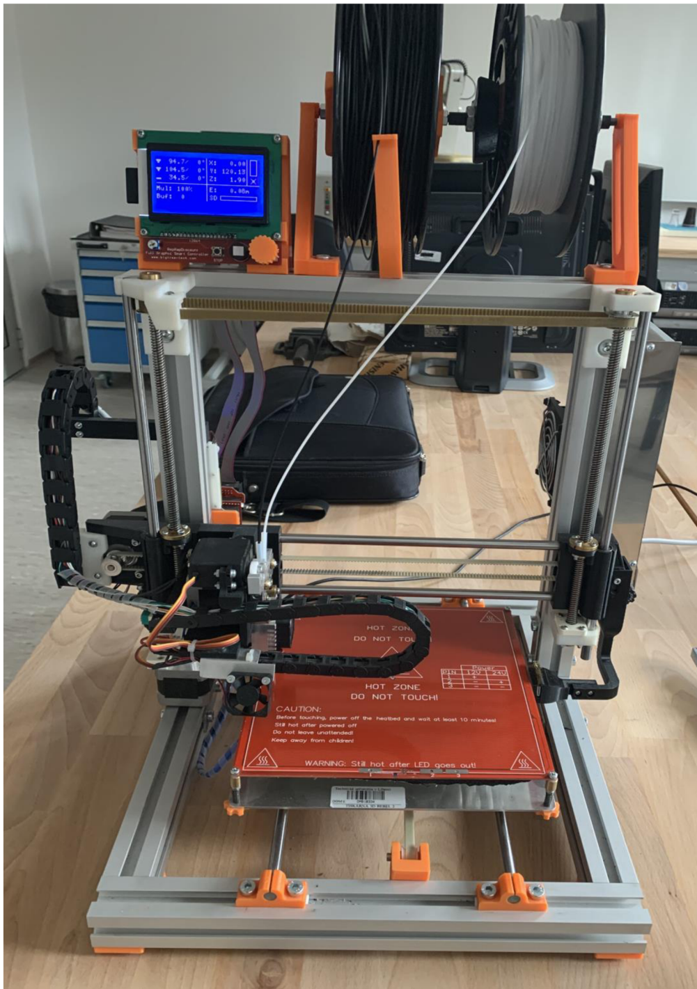
Figure 6: 3D Printer
