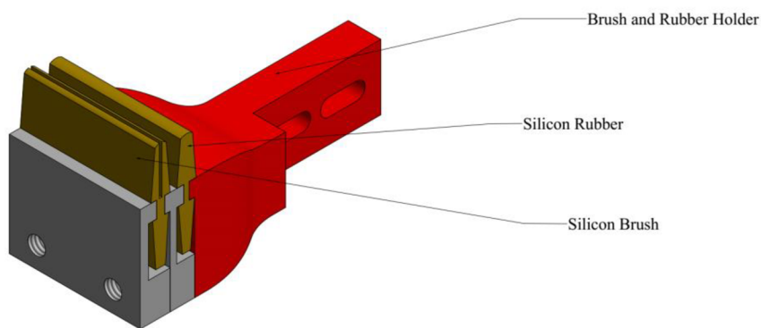
Figure 44: New Brush and Rubber Holder- 3D model
