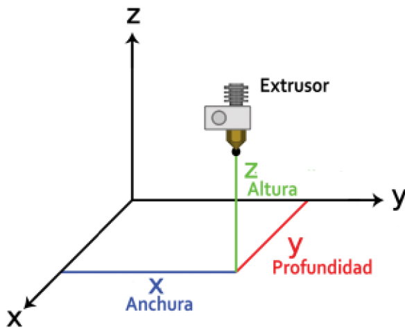
Figure 14: Cartesian Coordinate[8]
