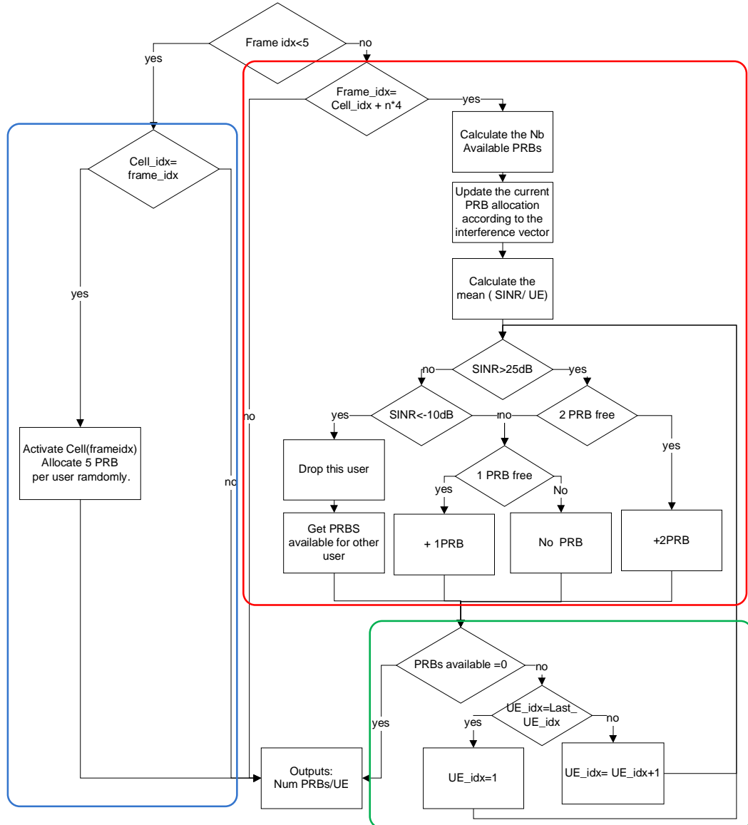
Figure 14: The SBA-A
