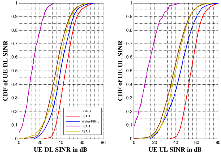
Figure 33: CDF SINR with fixed HeNBs
