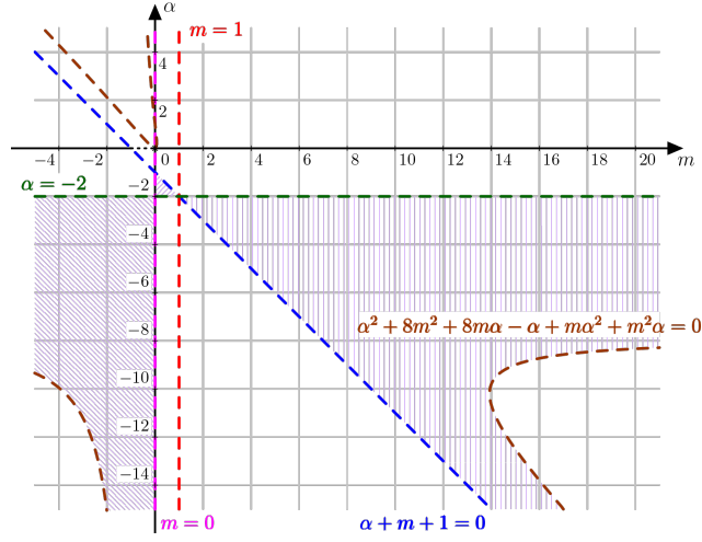
Figure 4.3: Summary of admissible values (Theorem 8)
