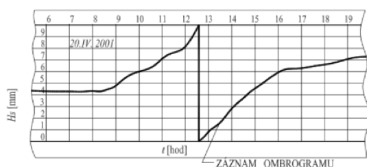
Obr. 4: Ombrogram (Starý, 2005)
