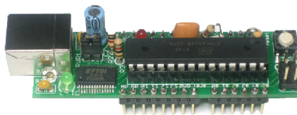
(b) Boarduino
