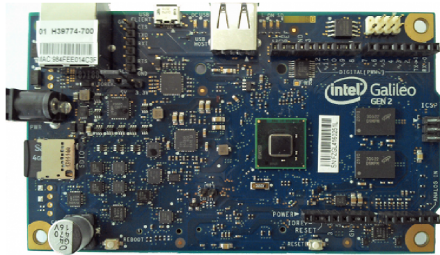
Obr. 2.14: Intel Galileo [35]
