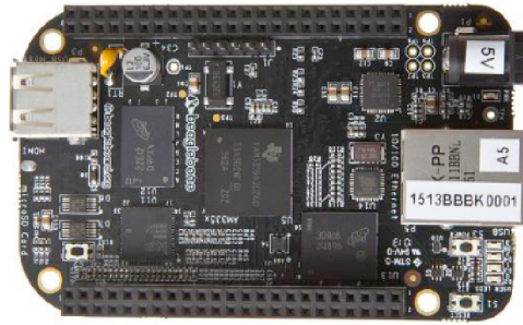
Obr. 2.13: BeagleBone Black [34]
