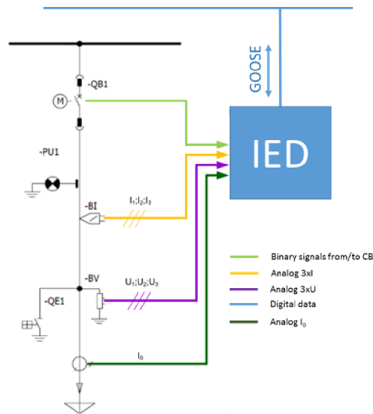
Fig. 7-3 : Typical incoming feeder with voltage measurement
