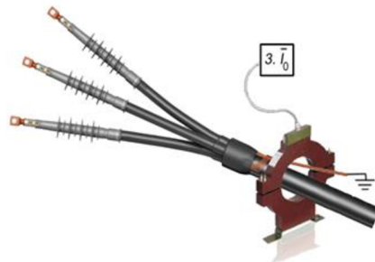
Fig. 6-1 : Example of core balance transformer
