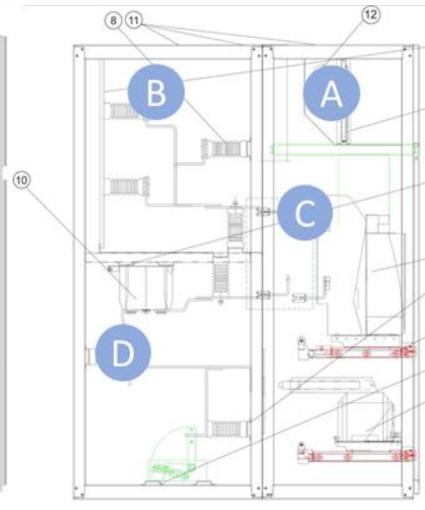
Fig. 2-2 : Cross section view Eaton 7.2kV Switchgear [9]
