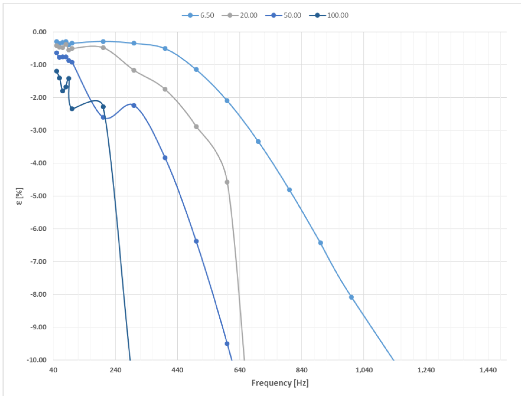
Fig. 5-7 : Frequency response of Resistive divider for various cable lengths
