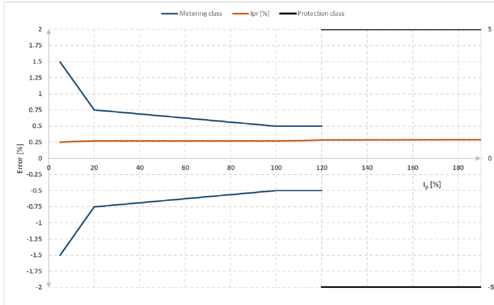
Fig. 3-4 : Combined accuracy limits of Rogowski coil at const. ambient temp. [23]
