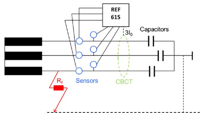
Fig. 6-9 : Block diagram – simulation of MV isolated neutral network
