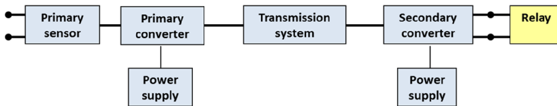
Fig. 5-1 : Definition of measurement accuracy chain according IEC 60044-8 [5]
