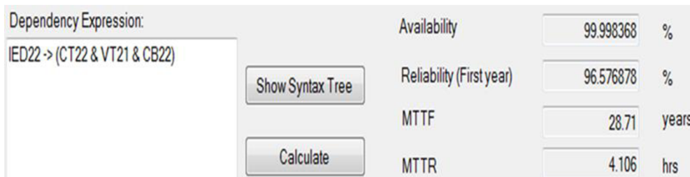
Fig. 7-10 : Reliability calculation results of PRP redundancy
