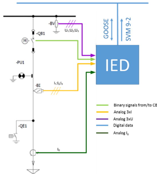
Fig. 7-4 : Typical outgoing feeder with busbar voltage measurement
