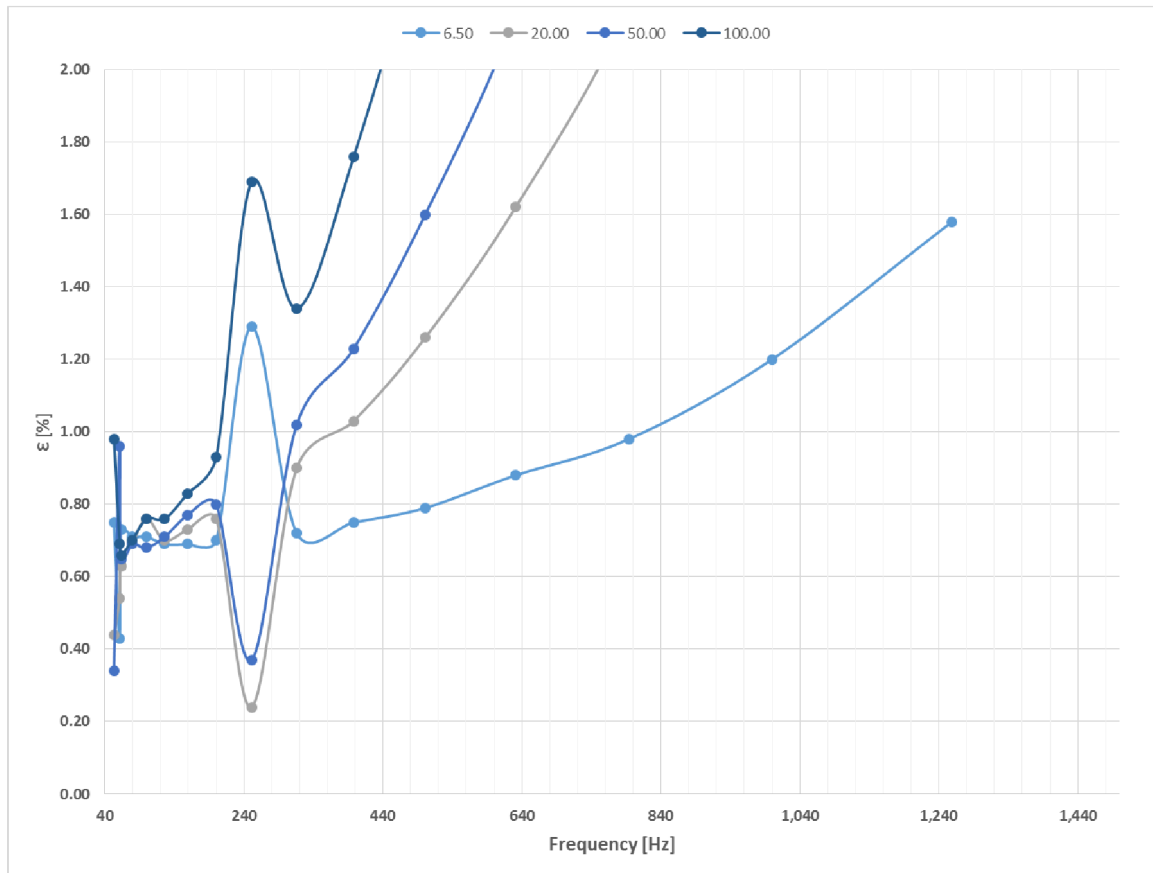
Fig. 5-5 : Frequency response of Rogowski for various cable lengths
