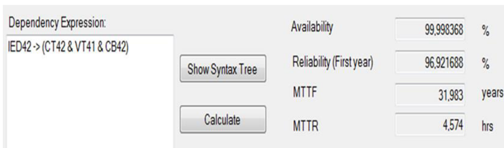
Fig. 7-11 : Reliability calculation results of HSR redundancy
