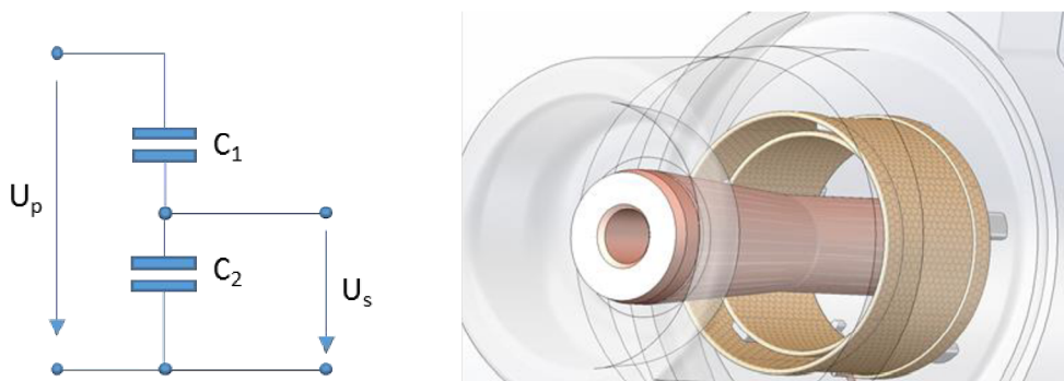
Fig. 3-7 : Left - capacitive divider scheme and Right – example of the assembly
