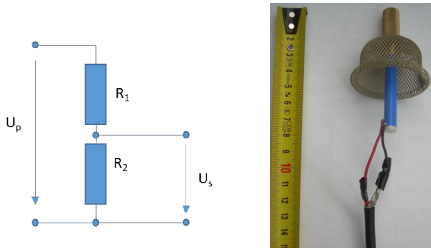
Fig. 3-6 : Left - Resistive divider scheme and Right – example of the assembly
