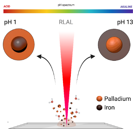
Figure 2.1: The proposed influence pH modification has on the element distribution in the final FePd nanoalloy synthesized using RLAL. Sketch created in BioRender.
