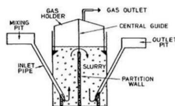
Fig 3. Floating drum biodigester (Ononogbo 2015)
