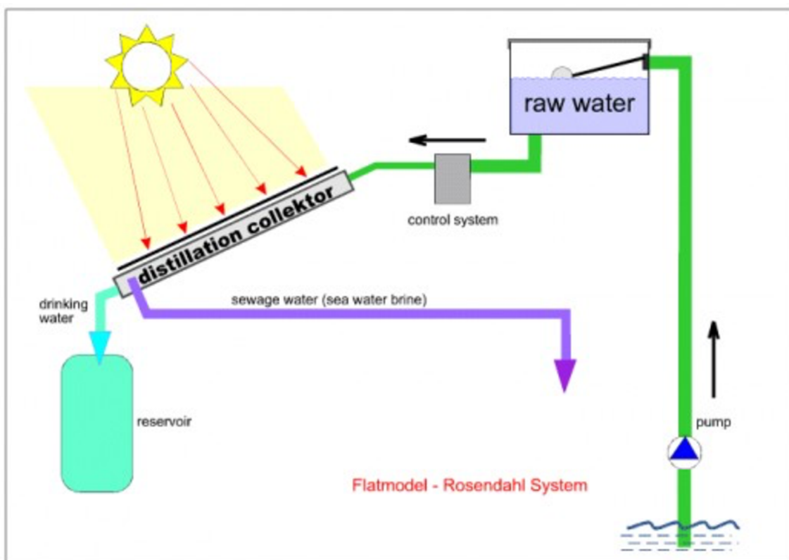
Figure 11 Solar Distillation
