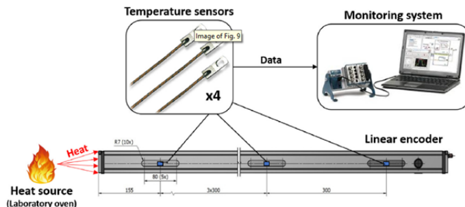
Obr. 4.8: Schéma experimentu [10]
