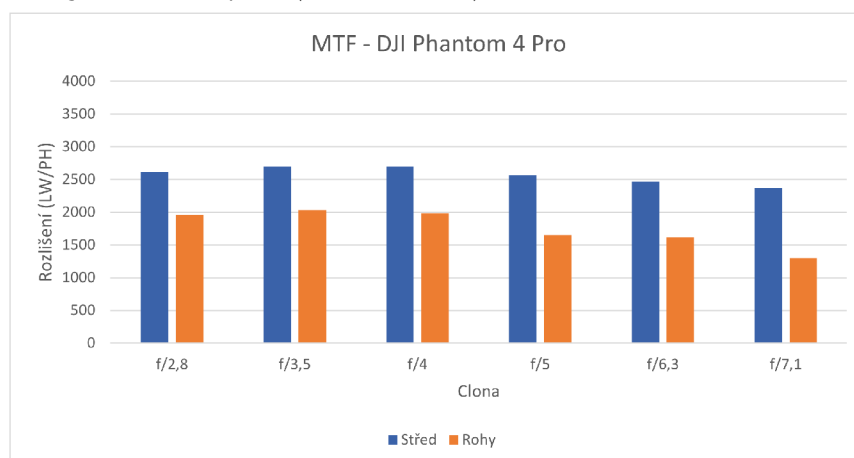
Obr. 4.3.3-12 Graf MTF dron DJI Phantom 4 Pro.
