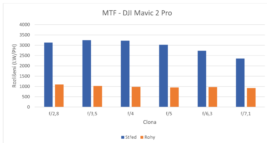
Obr. 4.3.3-13 Graf MTF dron DJI Mavic 2 Pro.
