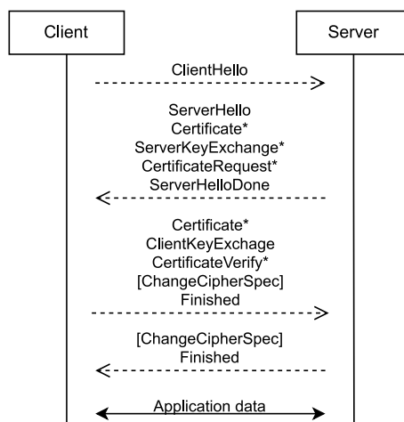
Fig. 1.2: TLS 1.2 full handshake
