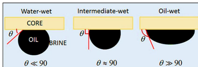
Figure 5 Schematic representation of the theory behind the estimation of the wettability behavior of reservoir rock when two immiscible phases exist (Omidi et al., 2020).
