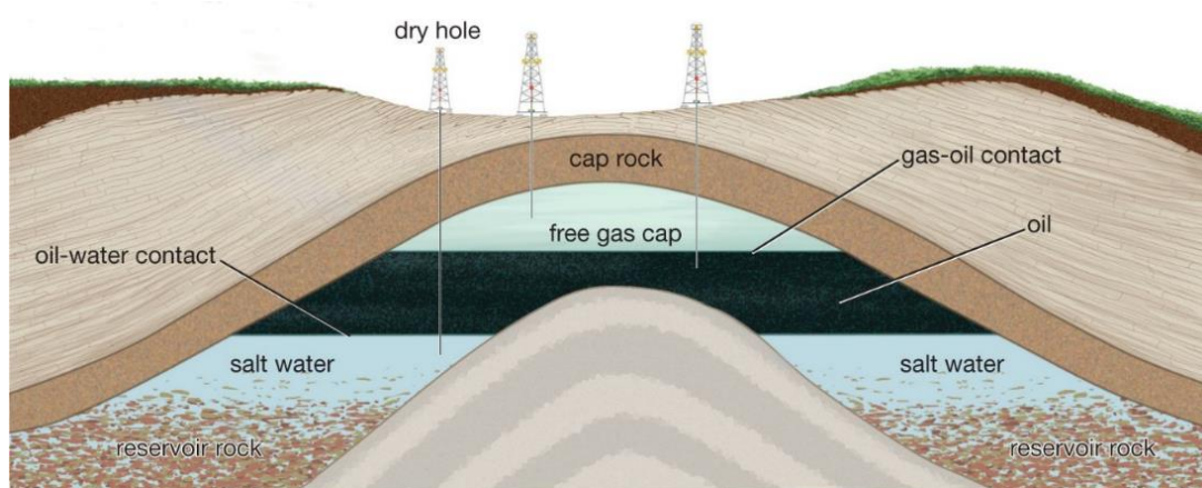
Figure 1 Petroleum reservoir (Druetta et al., 2016).
