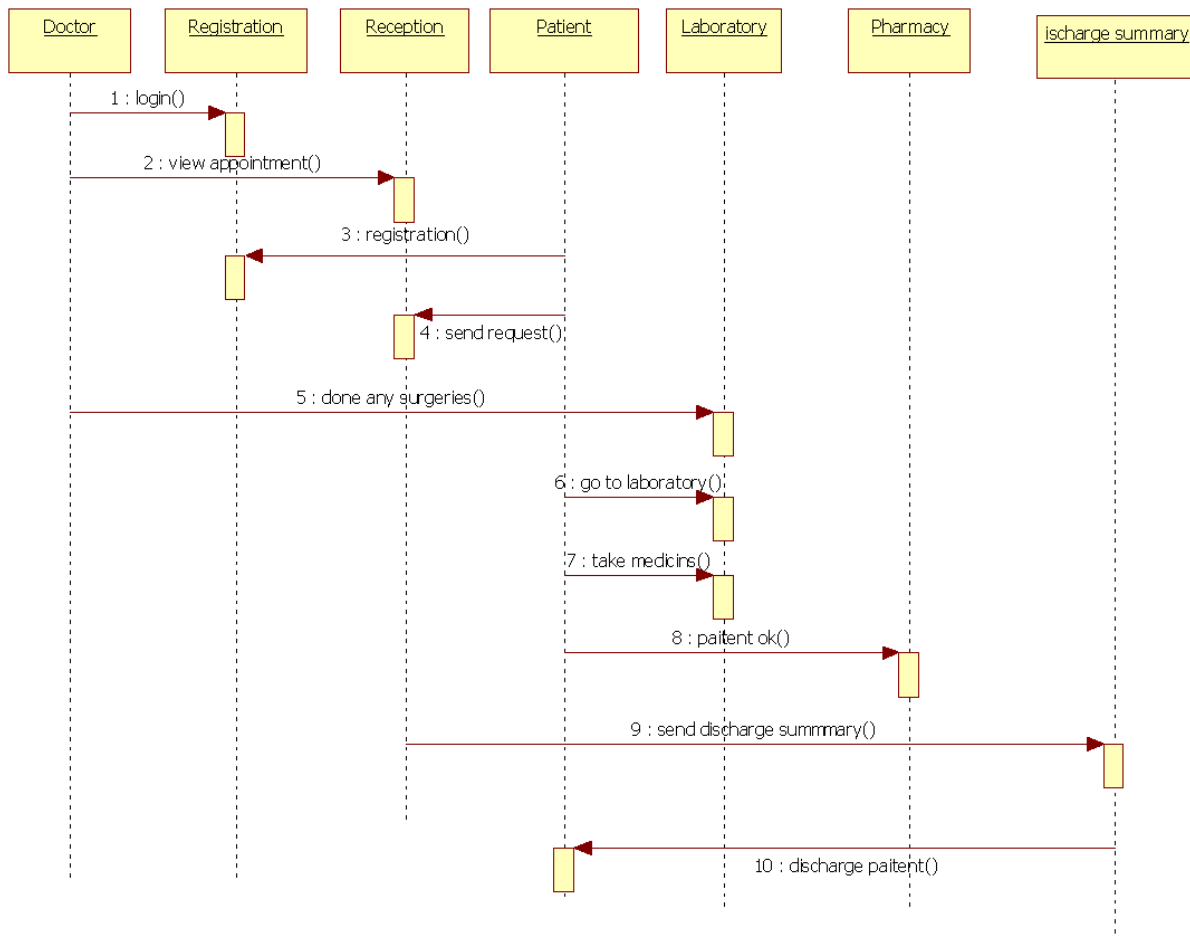
Figure 3 Sequence diagram
