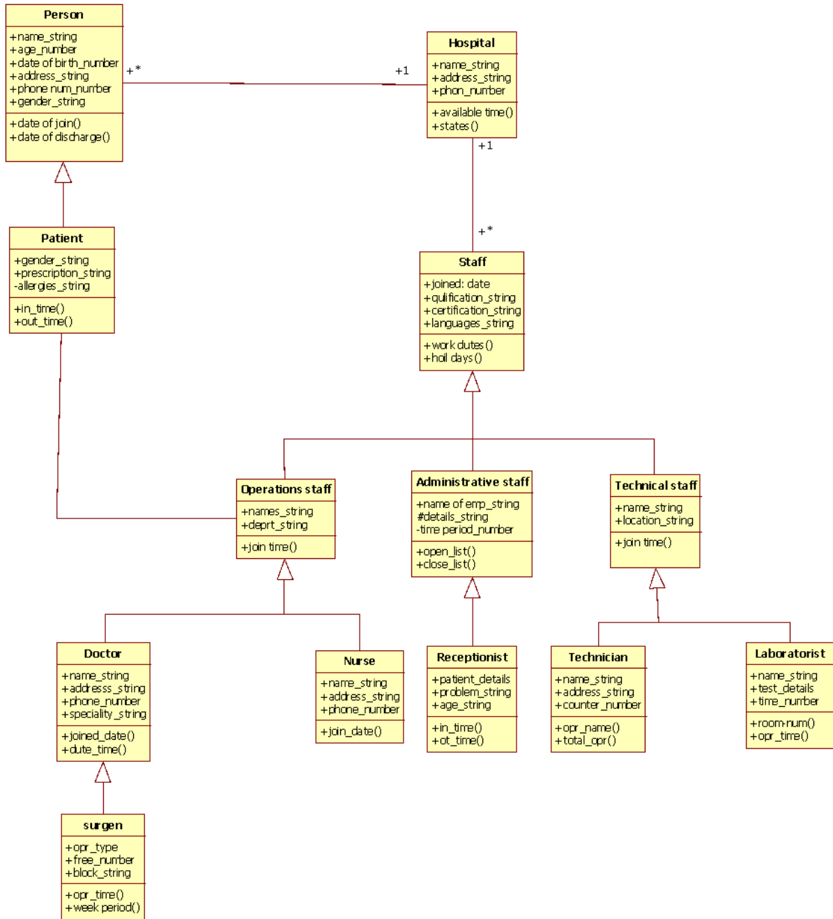
Figure 2 Class Diagram
