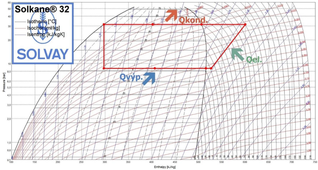
Obr. 24 P-H diagram okruhu TČ
