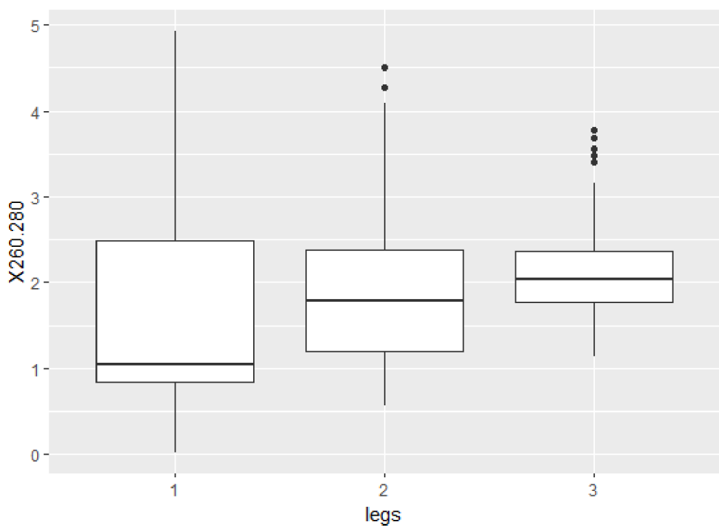
Figure 4. Number on the bottom in the x axis (legs) corresponds to the amount of leg tissue used for the extraction of DNA. Number on the left side in the y axis (X260.280) corresponds to the A260/A280 absorbance ratio.
