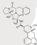
Ergotamin
