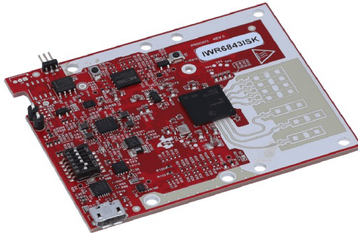
Obr. 3.12: Modul IWR6843ISK 5
