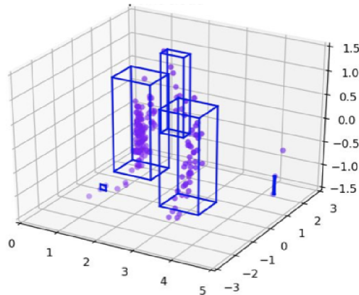
Obr. 3.9: Klastrovanie bodov 3
