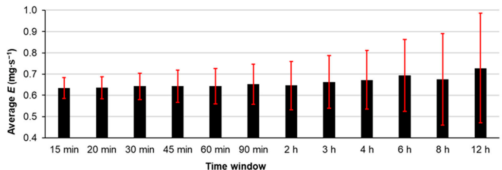
Figure 7. E dependence on the time window width for artificially modified model data (vertical red lines are standard deviation bars).
