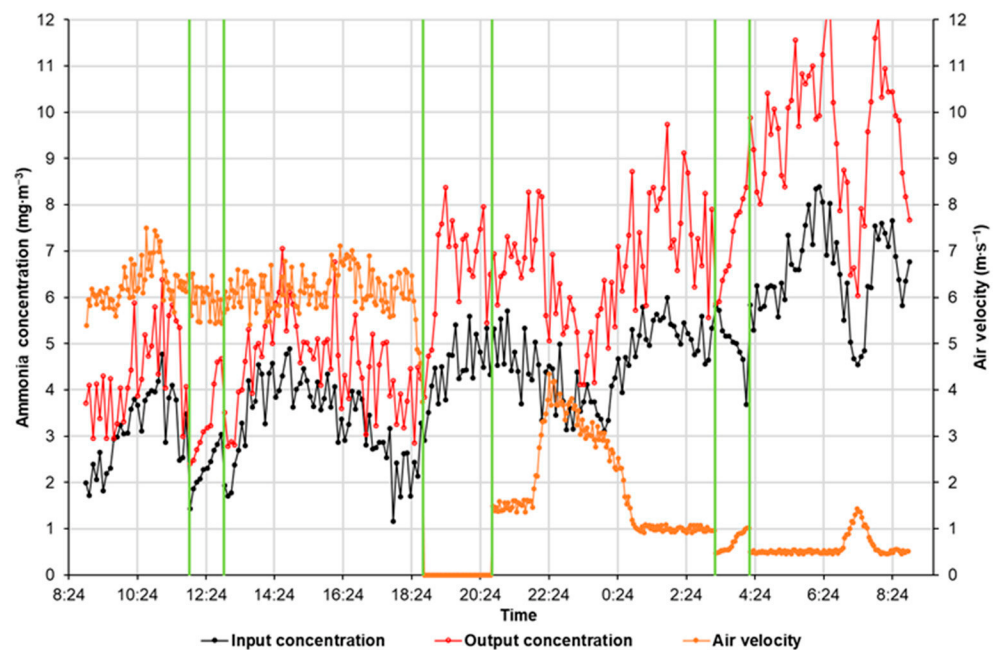
Figure 5. Creation of model values with randomly modified time intervals (three green gaps).
