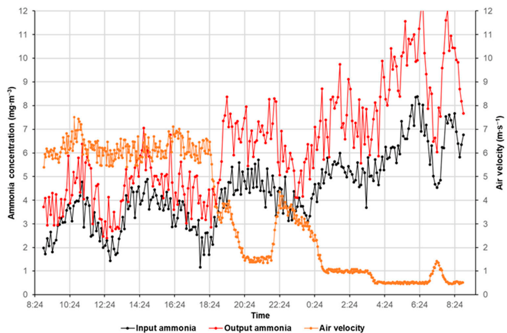
Figure 4. Creation of model values based on real data from the stable.
