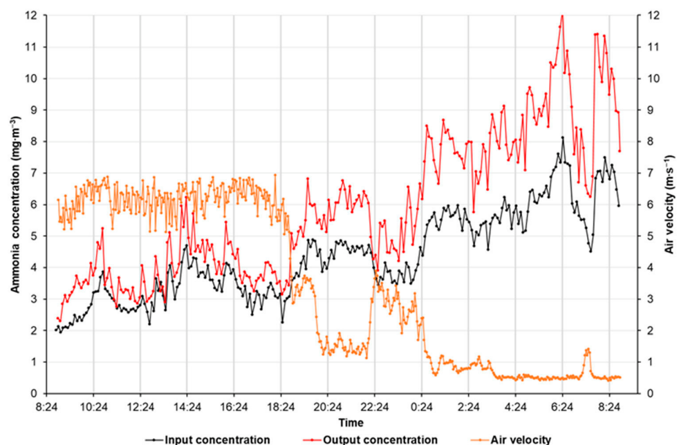
Figure 3. Measured data from experimental pig house.
