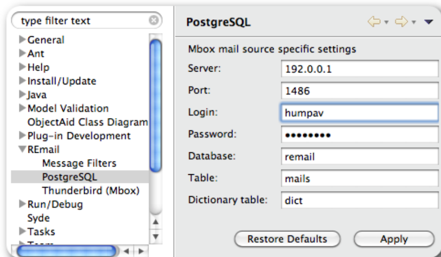
Figure 3.18: PostgreSQL preference page
