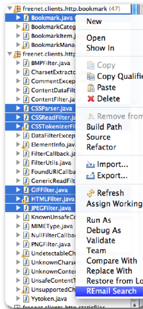
Figure 3.22: Starting search
