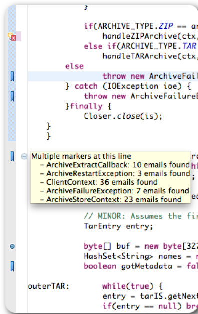
Figure 3.8: Using markers
