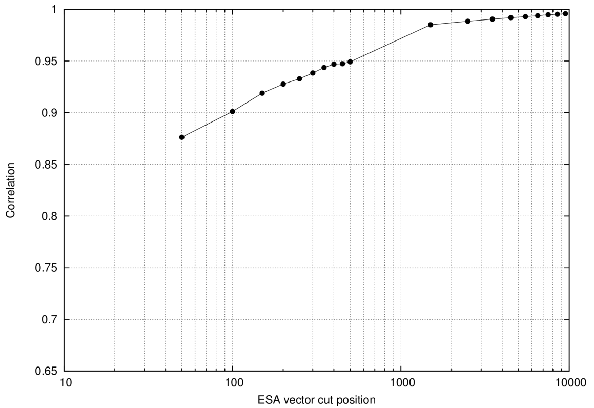
Figure 5.13: Half relevant, half randomly selected documents. The graph shows the relationship between correlation of the ranked document list (y-axis) and the ESA vector length (x-axis).
