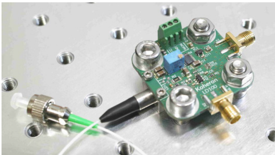
Obr. 4.10: Laser Koheron LD100 [20].
