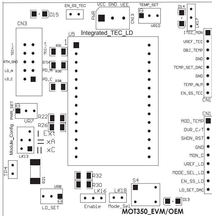
Obr. 4.3: Schéma modulu MOT350 [13].
